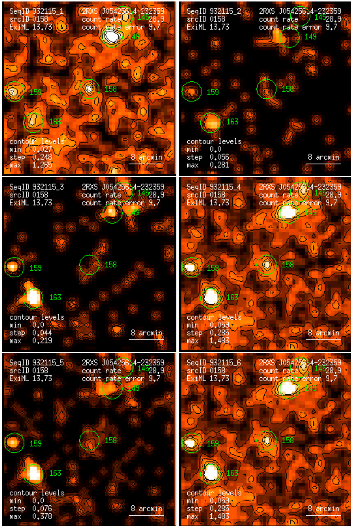
Figure 158: RASS 932115: detection 0158: band rate images, Gaussian filter: (1) PSPC channels 11 – 41, (2) 52 – 90, (3) 91 – 201, (4) 11 – 235, (5) 52 – 201, (6) 11 – 201. Broad band rates in counts/ks. Band rate contour levels in counts/ks/arcmin 2 .
