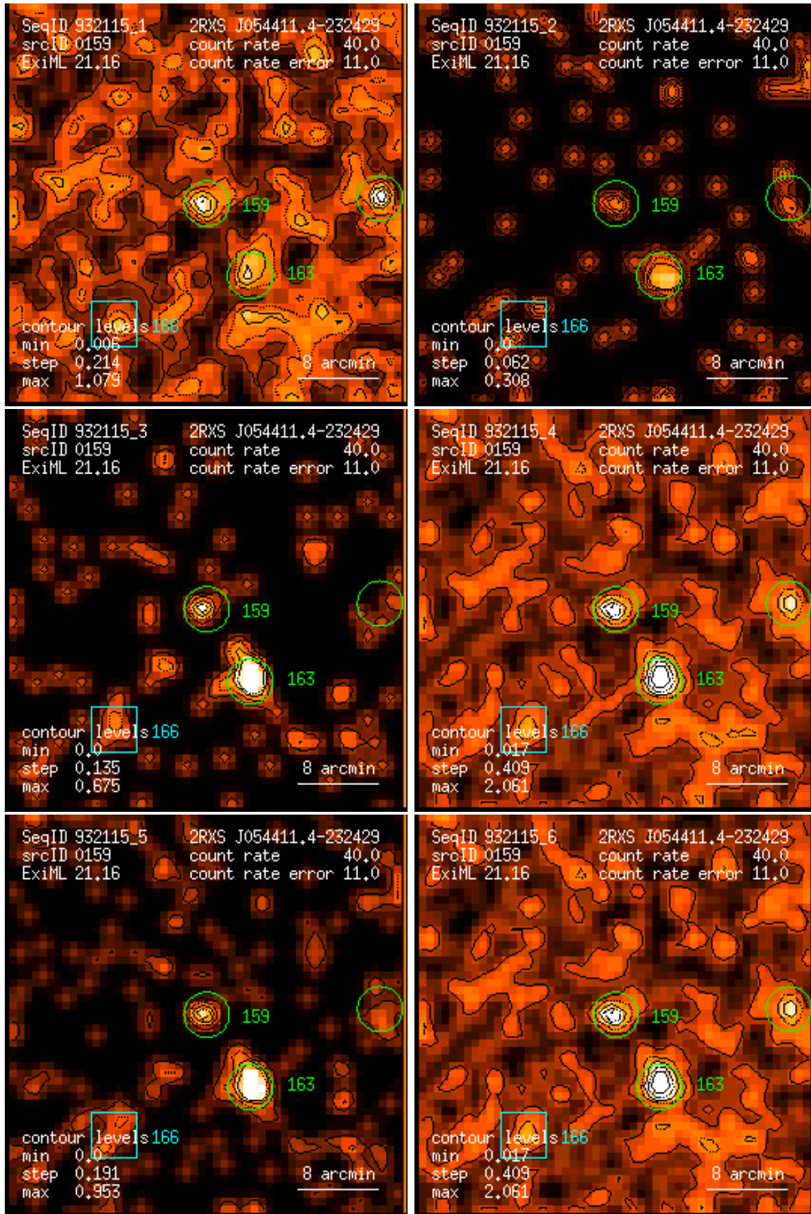
Figure 159: RASS 932115: detection 0159: band rate images, Gaussian filter: (1) PSPC channels 11 – 41, (2) 52 – 90, (3) 91 – 201, (4) 11 – 235, (5) 52 – 201, (6) 11 – 201. Broad band rates in counts/ks. Band rate contour levels in counts/ks/arcmin 2 .
