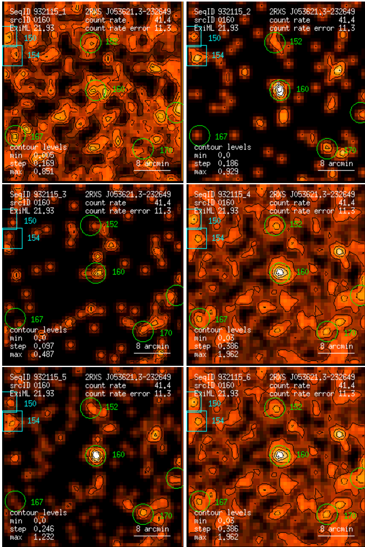
Figure 160: RASS 932115: detection 0160: band rate images, Gaussian filter: (1) PSPC channels 11 – 41, (2) 52 – 90, (3) 91 – 201, (4) 11 – 235, (5) 52 – 201, (6) 11 – 201. Broad band rates in counts/ks. Band rate contour levels in counts/ks/arcmin 2 .
