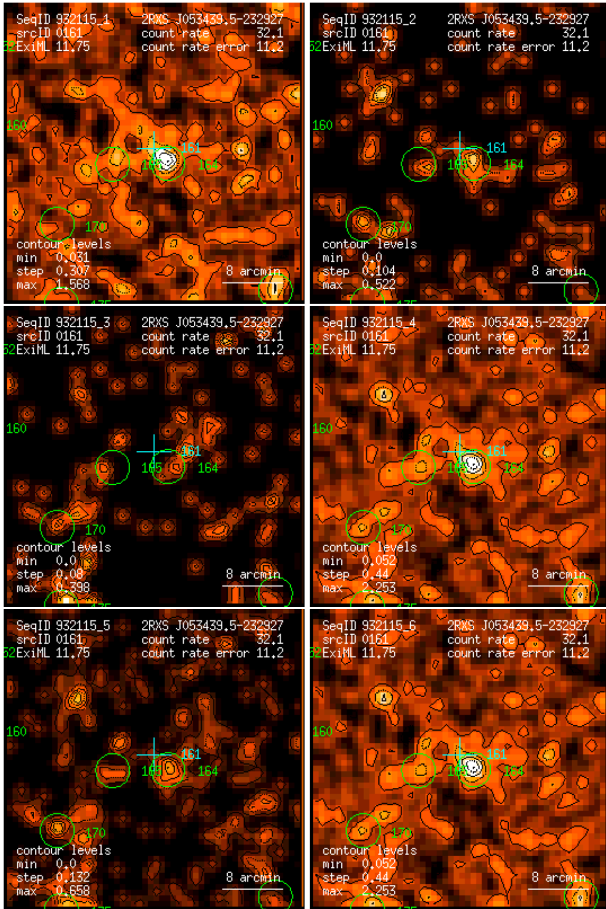
Figure 161: RASS 932115: detection 0161: band rate images, Gaussian filter: (1) PSPC channels 11 – 41, (2) 52 – 90, (3) 91 – 201, (4) 11 – 235, (5) 52 – 201, (6) 11 – 201. Broad band rates in counts/ks. Band rate contour levels in counts/ks/arcmin 2 .
