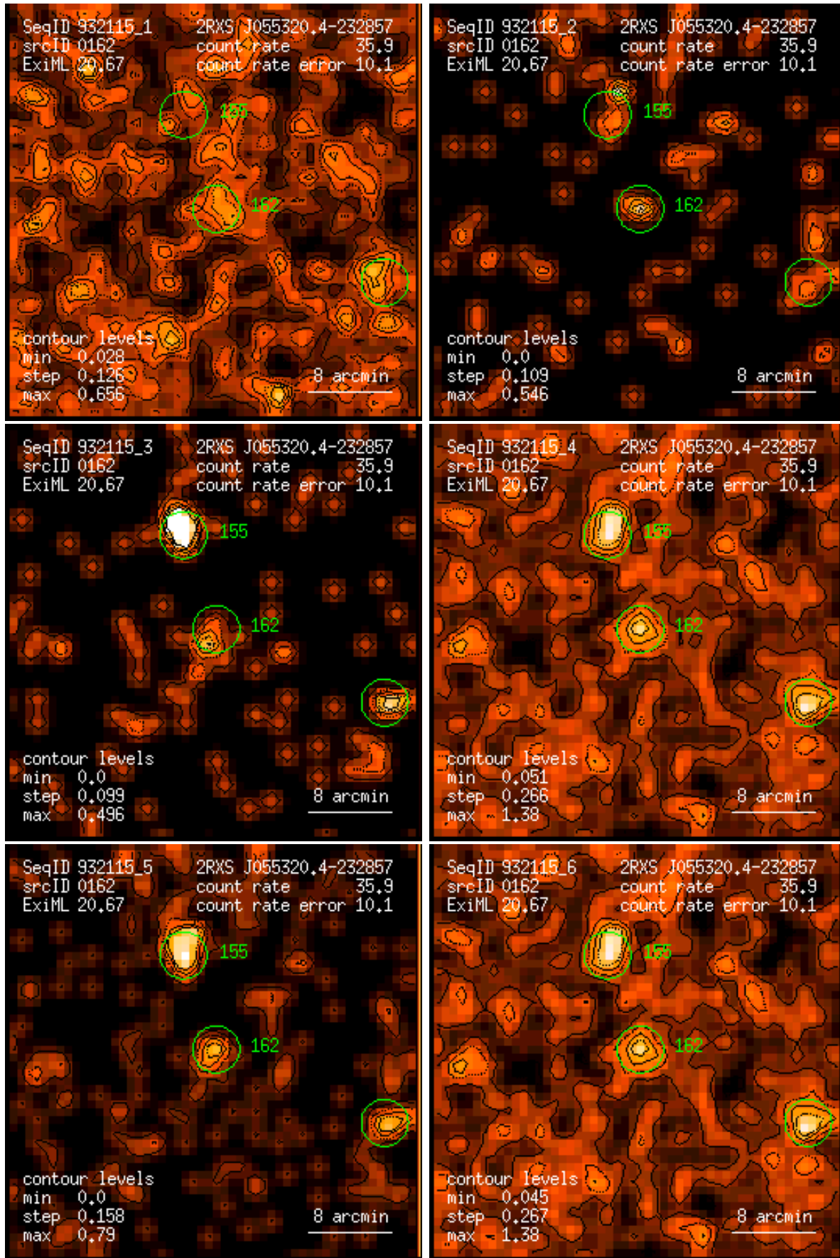
Figure 162: RASS 932115: detection 0162: band rate images, Gaussian filter: (1) PSPC channels 11 – 41, (2) 52 – 90, (3) 91 – 201, (4) 11 – 235, (5) 52 – 201, (6) 11 – 201. Broad band rates in counts/ks. Band rate contour levels in counts/ks/arcmin 2 .
