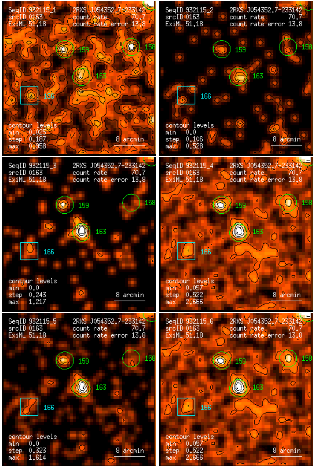
Figure 163: RASS 932115: detection 0163: band rate images, Gaussian filter: (1) PSPC channels 11 – 41, (2) 52 – 90, (3) 91 – 201, (4) 11 – 235, (5) 52 – 201, (6) 11 – 201. Broad band rates in counts/ks. Band rate contour levels in counts/ks/arcmin 2 .
