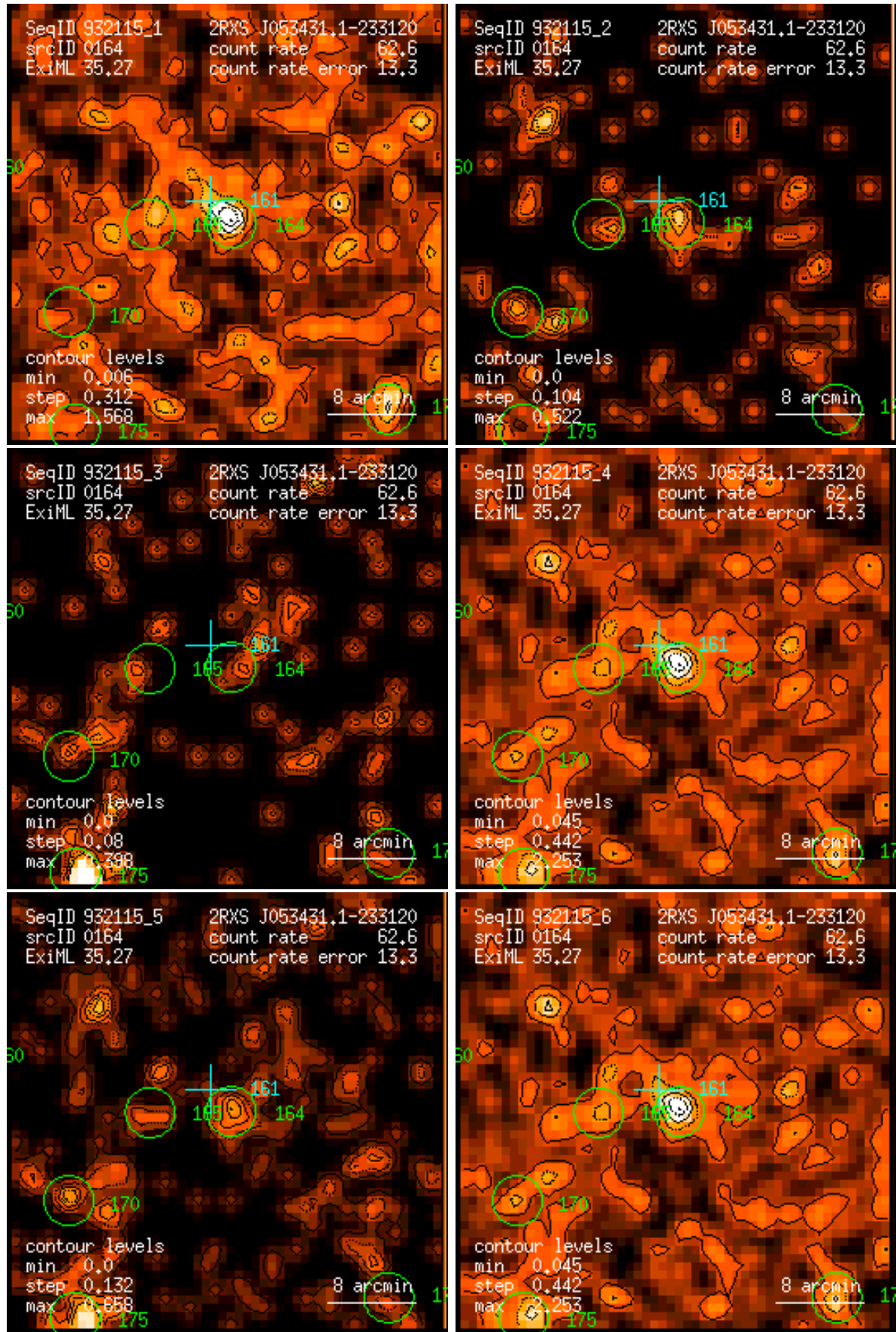
Figure 164: RASS 932115: detection 0164: band rate images, Gaussian filter: (1) PSPC channels 11 – 41, (2) 52 – 90, (3) 91 – 201, (4) 11 – 235, (5) 52 – 201, (6) 11 – 201. Broad band rates in counts/ks. Band rate contour levels in counts/ks/arcmin 2 .
