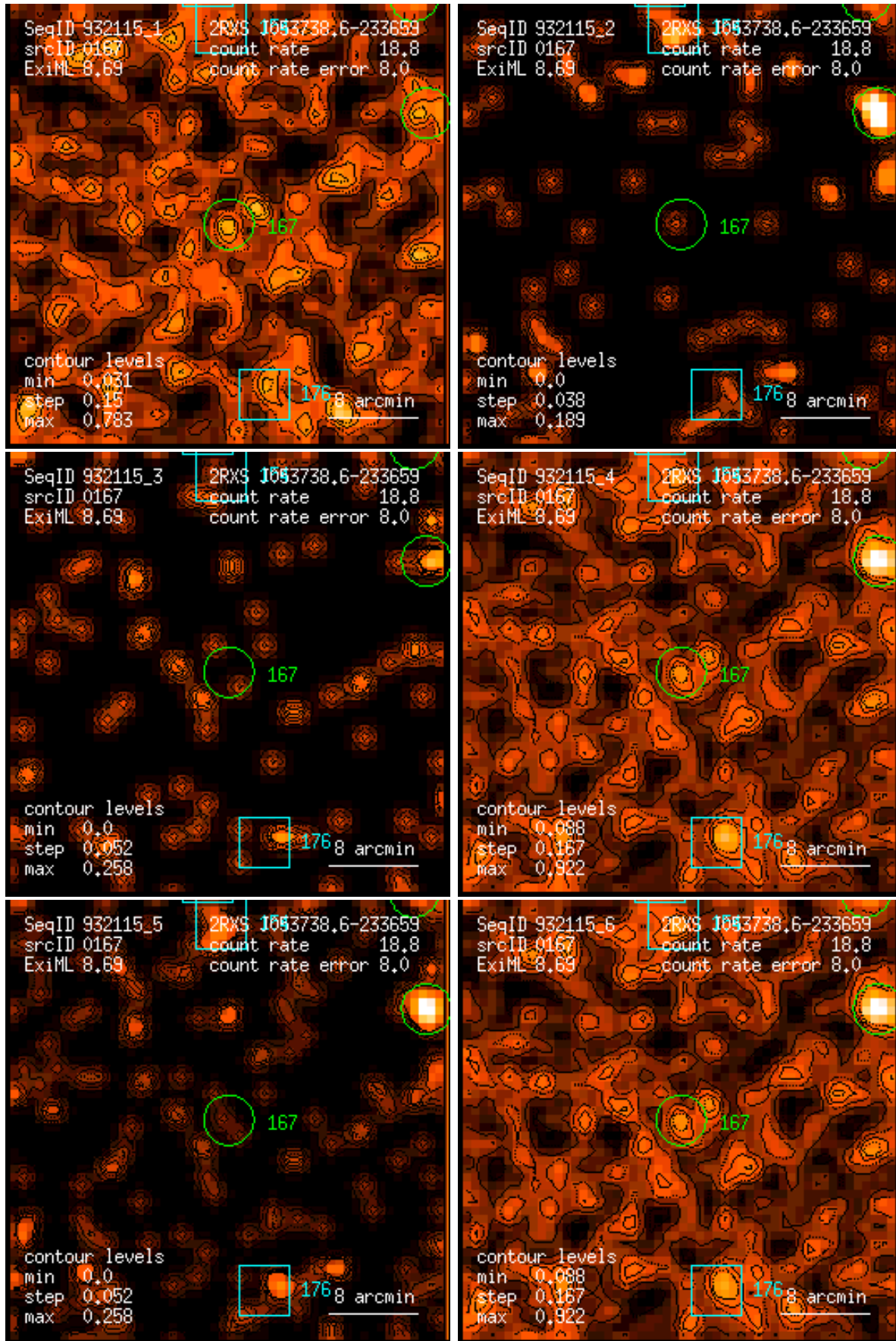
Figure 167: RASS 932115: detection 0167: band rate images, Gaussian filter: (1) PSPC channels 11 – 41, (2) 52 – 90, (3) 91 – 201, (4) 11 – 235, (5) 52 – 201, (6) 11 – 201. Broad band rates in counts/ks. Band rate contour levels in counts/ks/arcmin 2 .
