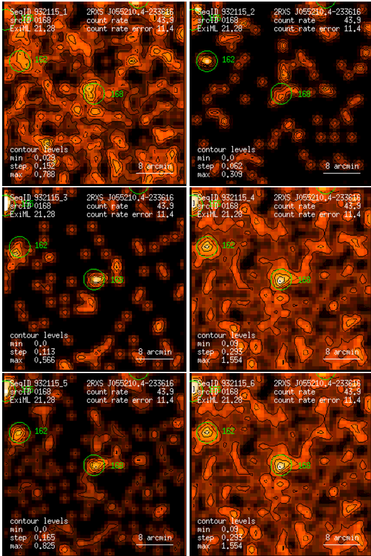
Figure 168: RASS 932115: detection 0168: band rate images, Gaussian filter: (1) PSPC channels 11 – 41, (2) 52 – 90, (3) 91 – 201, (4) 11 – 235, (5) 52 – 201, (6) 11 – 201. Broad band rates in counts/ks. Band rate contour levels in counts/ks/arcmin 2 .
