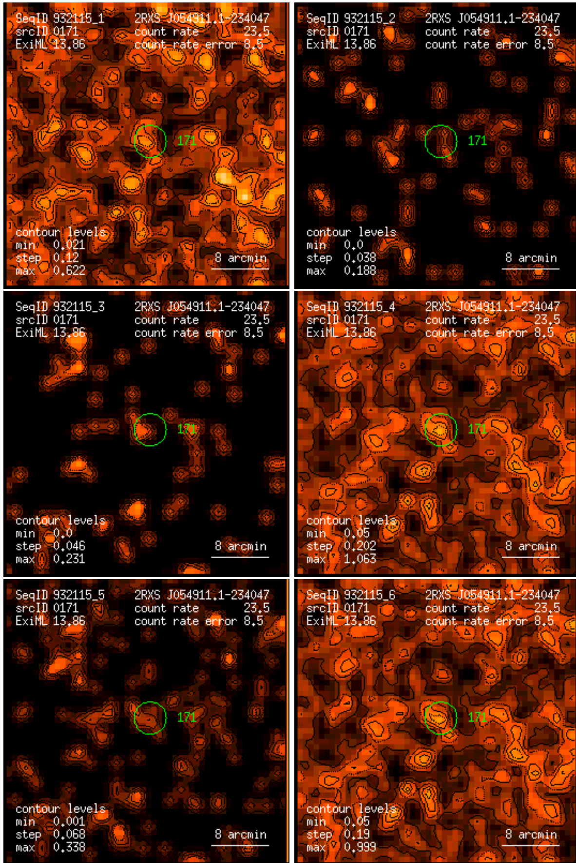
Figure 171: RASS 932115: detection 0171: band rate images, Gaussian filter: (1) PSPC channels 11 – 41, (2) 52 – 90, (3) 91 – 201, (4) 11 – 235, (5) 52 – 201, (6) 11 – 201. Broad band rates in counts/ks. Band rate contour levels in counts/ks/arcmin 2 .
