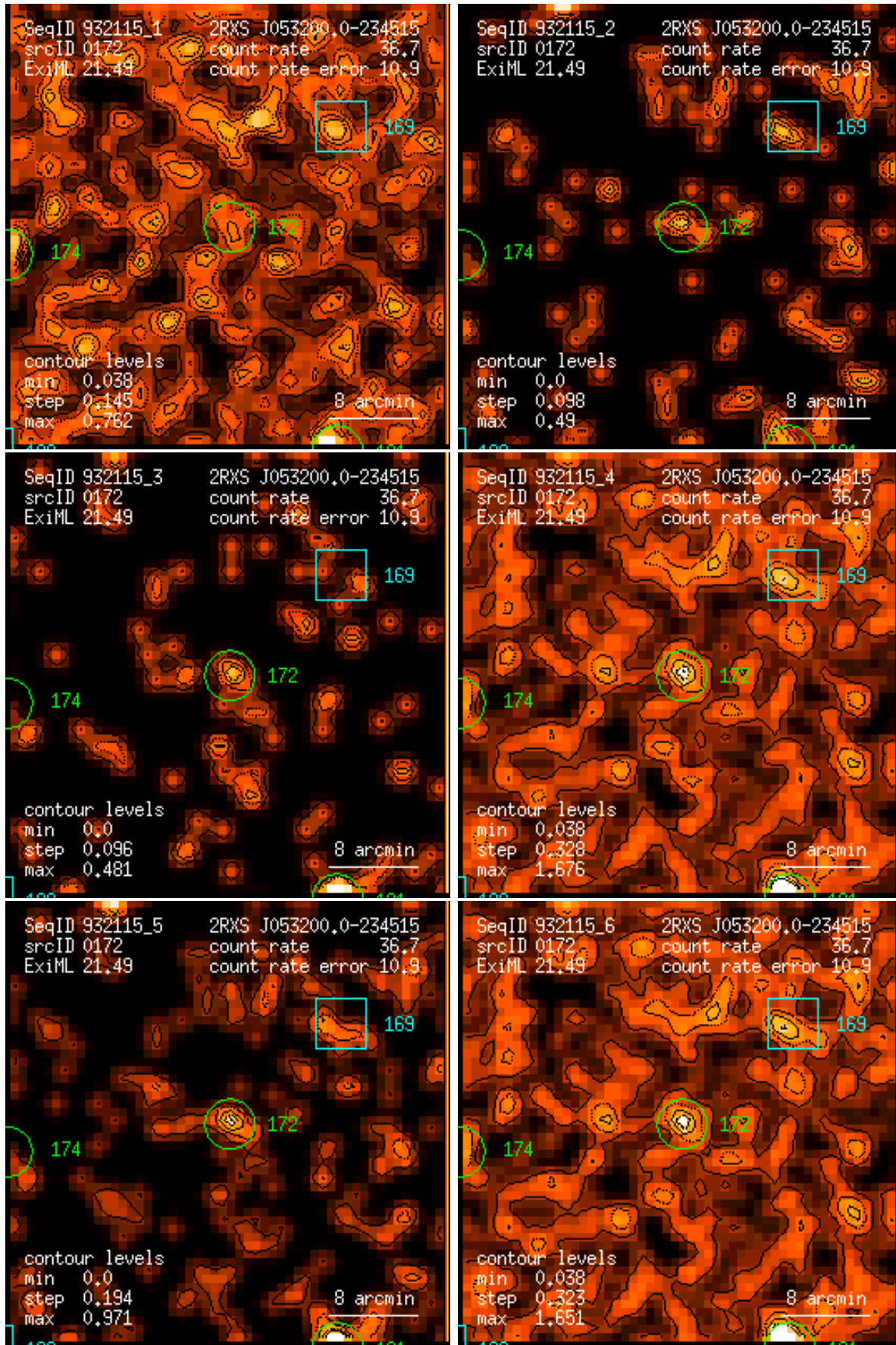
Figure 172: RASS 932115: detection 0172: band rate images, Gaussian filter: (1) PSPC channels 11 – 41, (2) 52 – 90, (3) 91 – 201, (4) 11 – 235, (5) 52 – 201, (6) 11 – 201. Broad band rates in counts/ks. Band rate contour levels in counts/ks/arcmin 2 .
