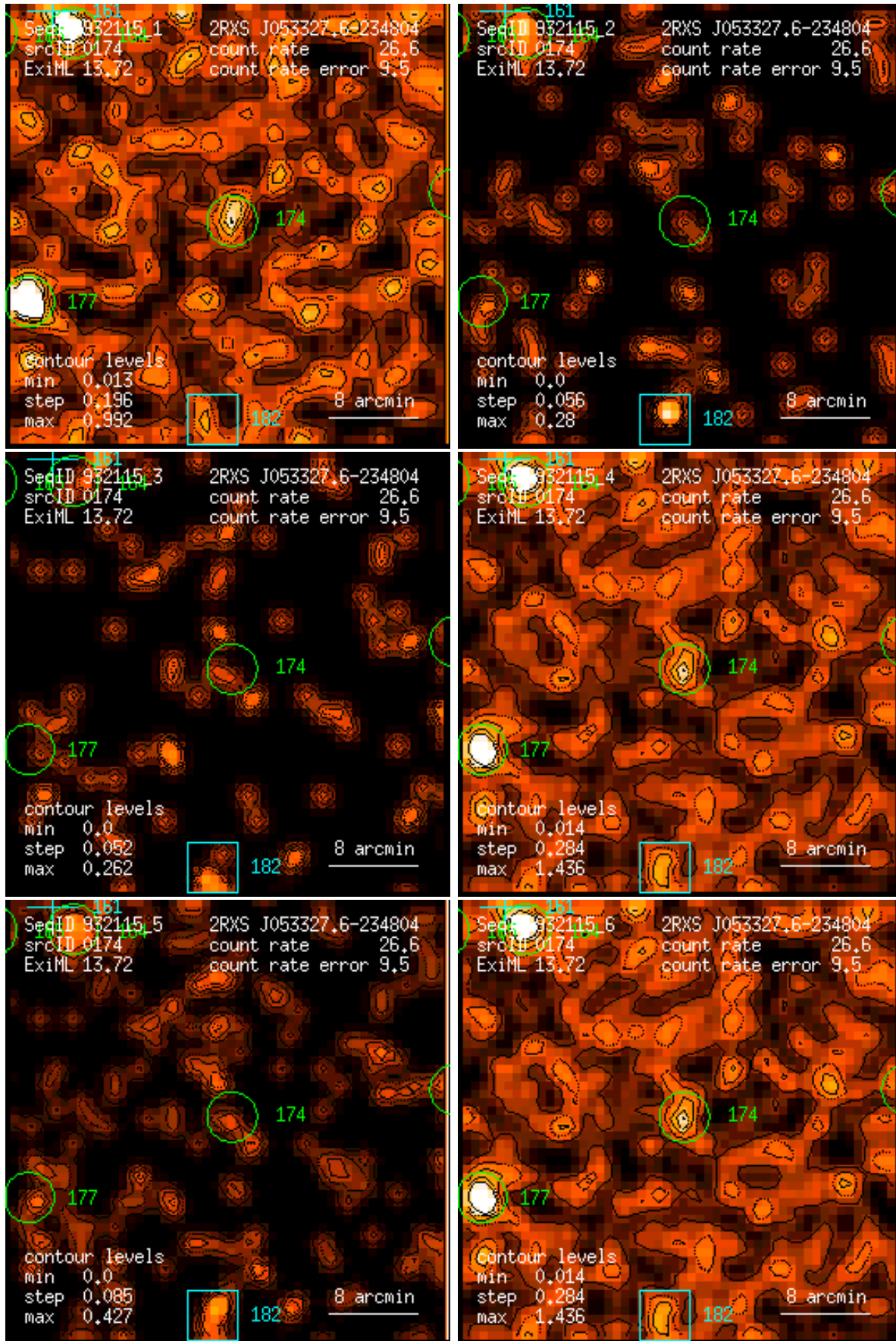
Figure 174: RASS 932115: detection 0174: band rate images, Gaussian filter: (1) PSPC channels 11 – 41, (2) 52 – 90, (3) 91 – 201, (4) 11 – 235, (5) 52 – 201, (6) 11 – 201. Broad band rates in counts/ks. Band rate contour levels in counts/ks/arcmin 2 .
