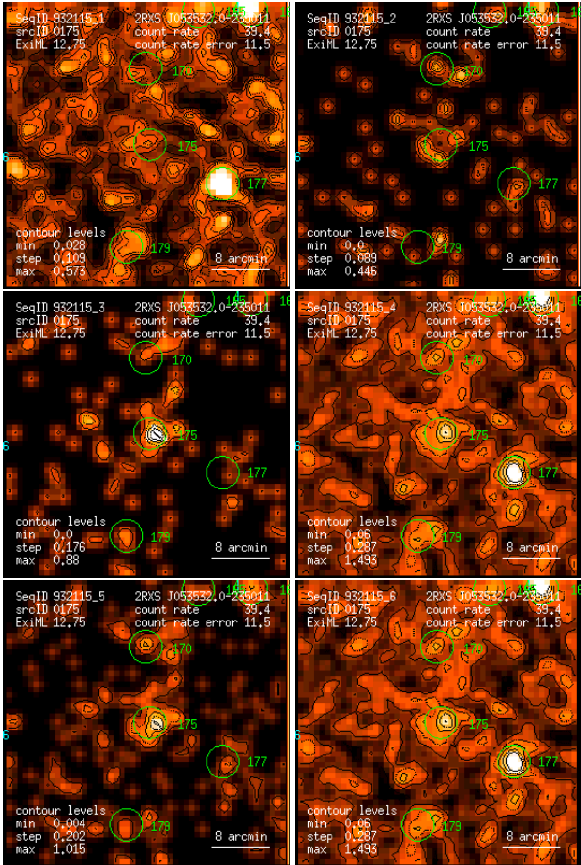
Figure 175: RASS 932115: detection 0175: band rate images, Gaussian filter: (1) PSPC channels 11 – 41, (2) 52 – 90, (3) 91 – 201, (4) 11 – 235, (5) 52 – 201, (6) 11 – 201. Broad band rates in counts/ks. Band rate contour levels in counts/ks/arcmin 2 .
