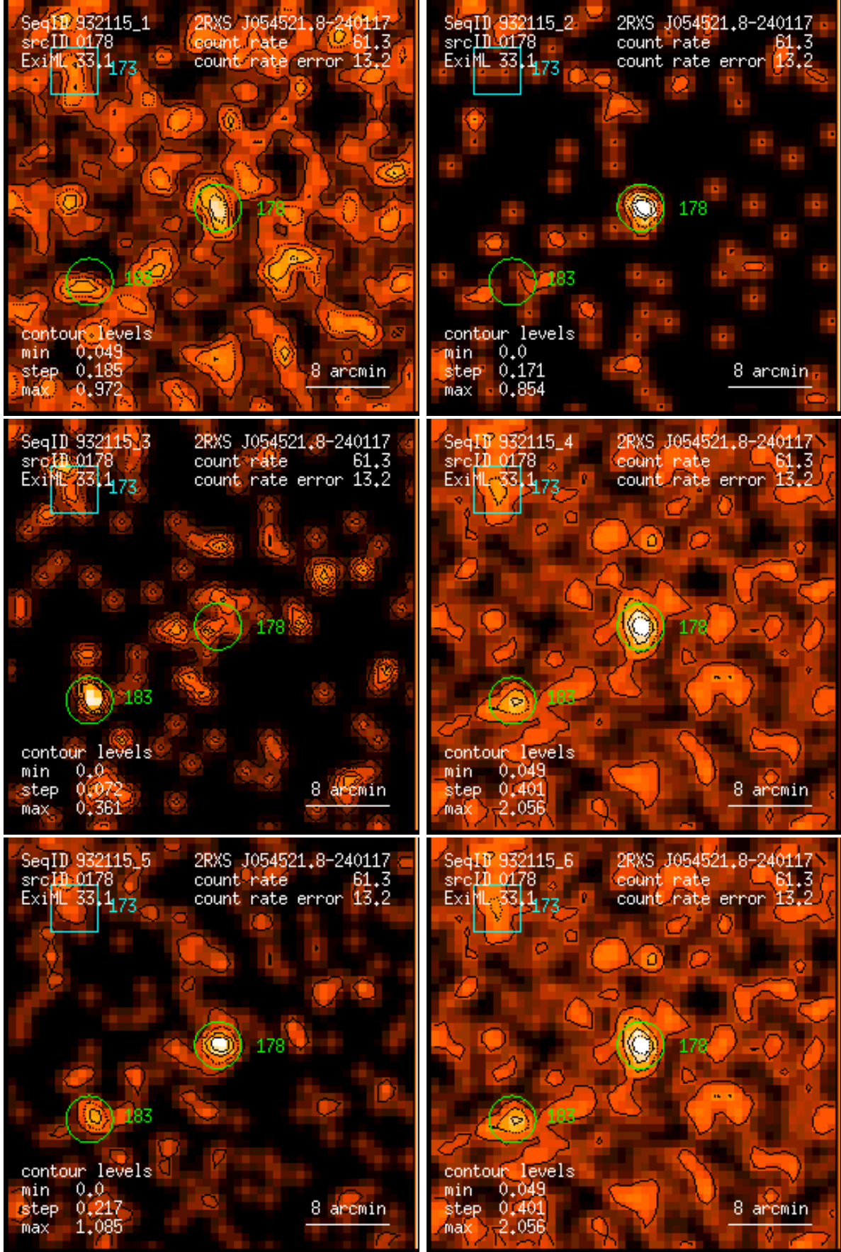
Figure 178: RASS 932115: detection 0178: band rate images, Gaussian filter: (1) PSPC channels 11 – 41, (2) 52 – 90, (3) 91 – 201, (4) 11 – 235, (5) 52 – 201, (6) 11 – 201. Broad band rates in counts/ks. Band rate contour levels in counts/ks/arcmin 2 .
