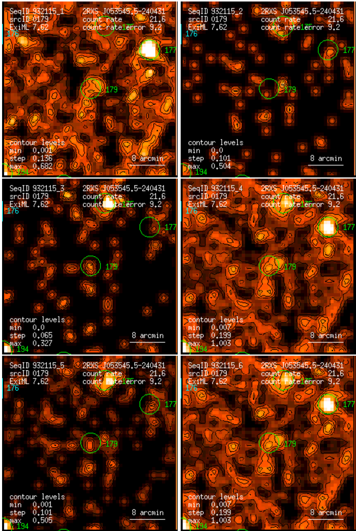
Figure 179: RASS 932115: detection 0179: band rate images, Gaussian filter: (1) PSPPC channels 11 – 41, (2) 52 – 90, (3) 91 – 201, (4) 11 – 235, (5) 52 – 201, (6) 11 – 201. Broad band rates in counts/ks. Band rate contour levels in counts/ks/arcmin 2 .
