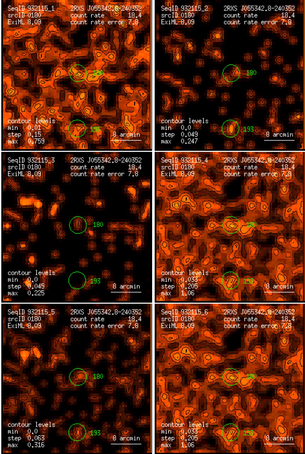
Figure 180: RASS 932115: detection 0180: band rate images, Gaussian filter: (1) PSPC channels 11 – 41, (2) 52 – 90, (3) 91 – 201, (4) 11 – 235, (5) 52 – 201, (6) 11 – 201. Broad band rates in counts/ks. Band rate contour levels in counts/ks/arcmin 2 .
