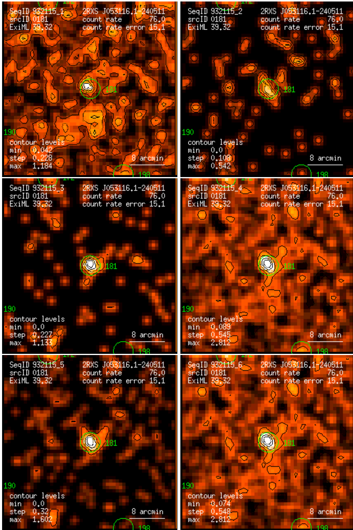
Figure 181: RASS 932115: detection 0181: band rate images, Gaussian filter: (1) PSPC channels 11 – 41, (2) 52 – 90, (3) 91 – 201, (4) 11 – 235, (5) 52 – 201, (6) 11 – 201. Broad band rates in counts/ks. Band rate contour levels in counts/ks/arcmin 2 .
