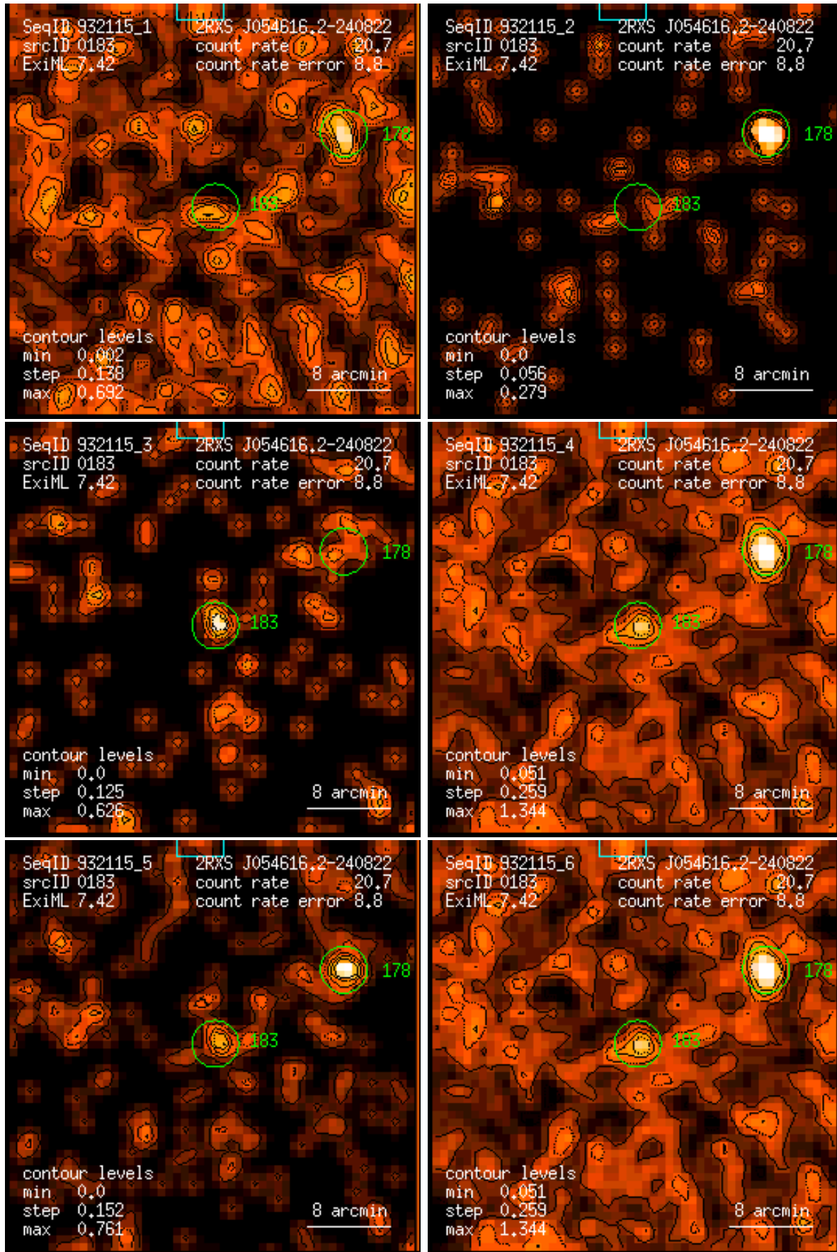
Figure 183: RASS 932115: detection 0183: band rate images, Gaussian filter: (1) PSPC channels 11 – 41, (2) 52 – 90, (3) 91 – 201, (4) 11 – 235, (5) 52 – 201, (6) 11 – 201. Broad band rates in counts/ks. Band rate contour levels in counts/ks/arcmin 2 .
