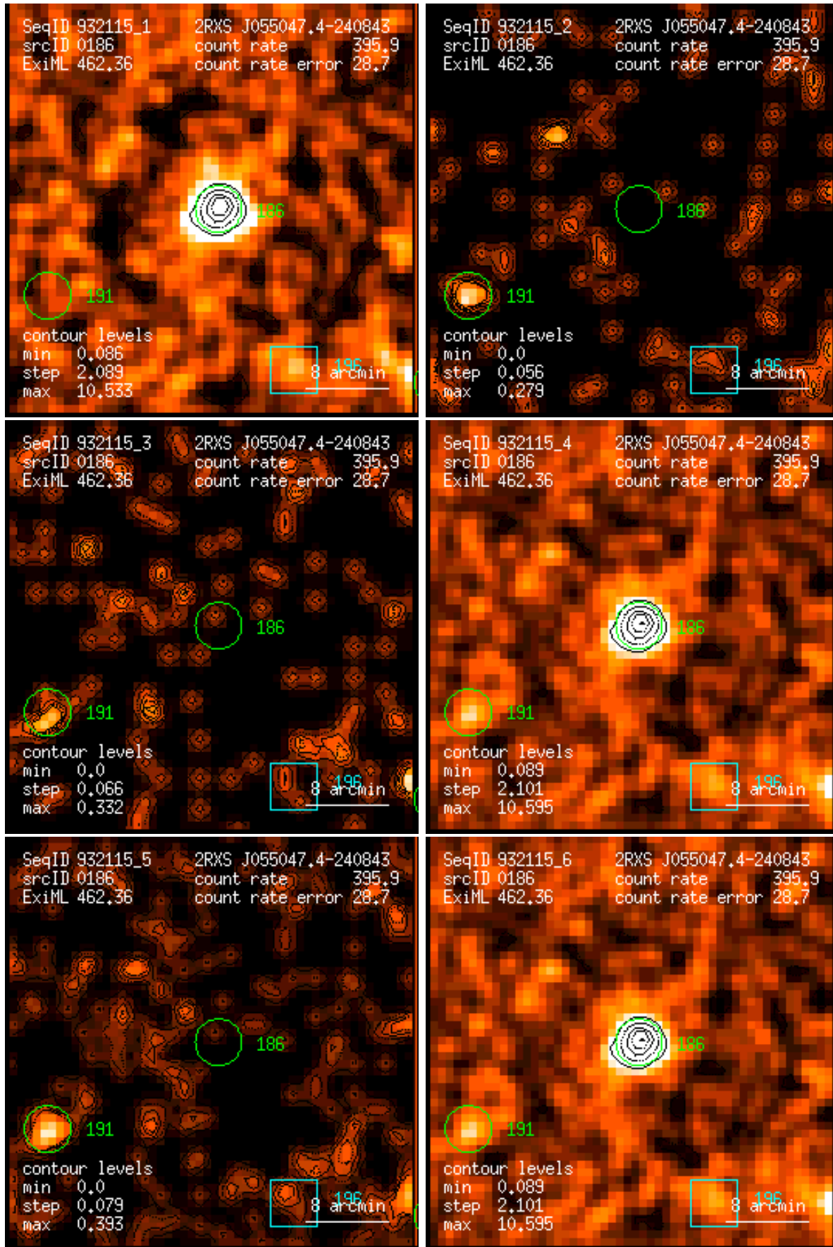
Figure 186: RASS 932115: detection 0186: band rate images, Gaussian filter: (1) PSPC channels 11 – 41, (2) 52 – 90, (3) 91 – 201, (4) 11 – 235, (5) 52 – 201, (6) 11 – 201. Broad band rates in counts/ks. Band rate contour levels in counts/ks/arcmin 2 .
