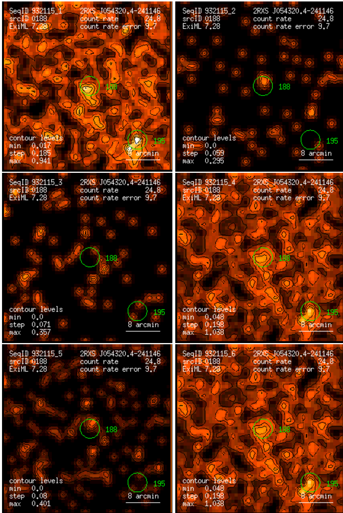
Figure 188: RASS 932115: detection 0188: band rate images, Gaussian filter: (1) PSPC channels 11 – 41, (2) 52 – 90, (3) 91 – 201, (4) 11 – 235, (5) 52 – 201, (6) 11 – 201. Broad band rates in counts/ks. Band rate contour levels in counts/ks/arcmin 2 .
