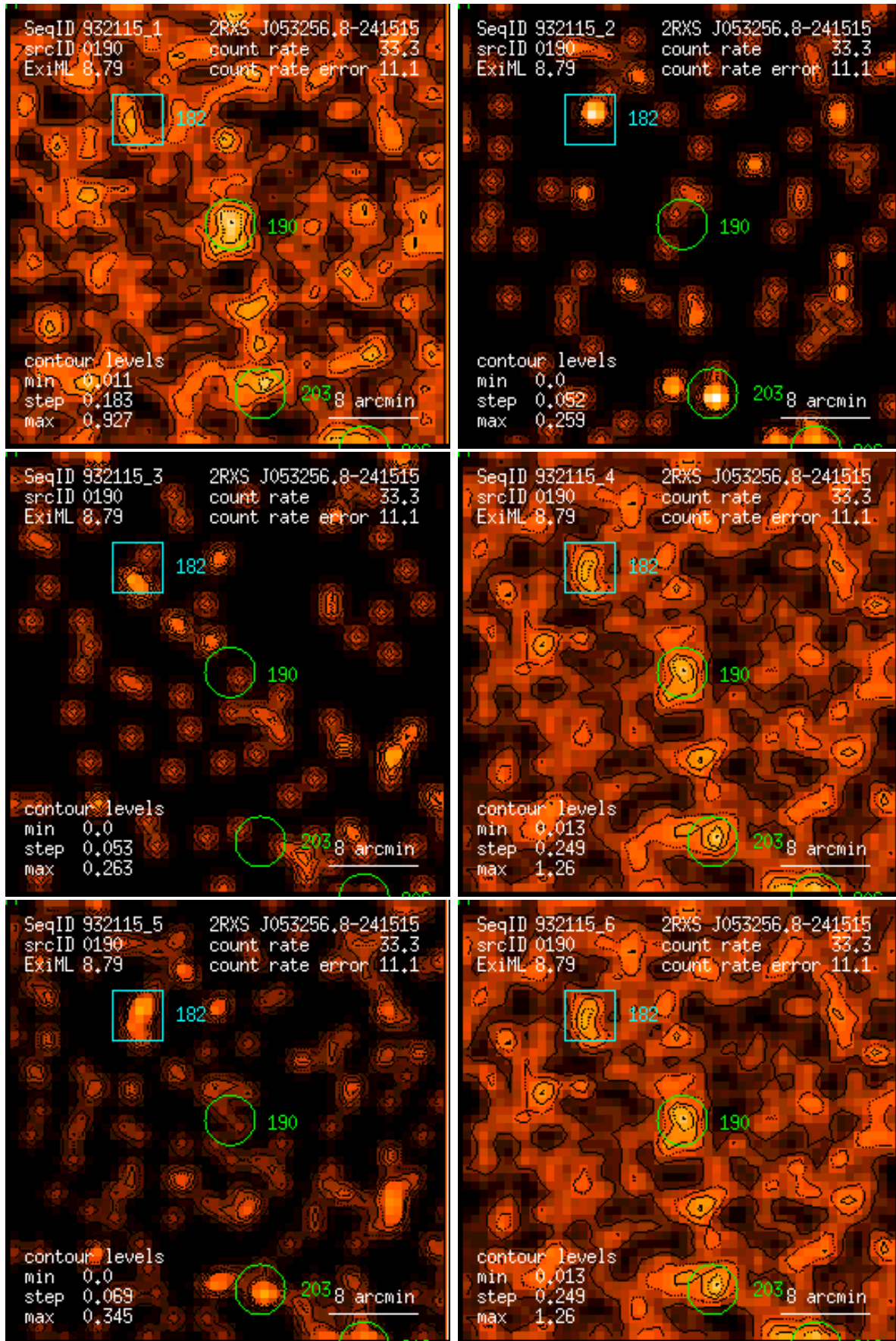
Figure 190: RASS 932115: detection 0190: band rate images, Gaussian filter: (1) PSPC channels 11 – 41, (2) 52 – 90, (3) 91 – 201, (4) 11 – 235, (5) 52 – 201, (6) 11 – 201. Broad band rates in counts/ks. Band rate contour levels in counts/ks/arcmin 2 .
