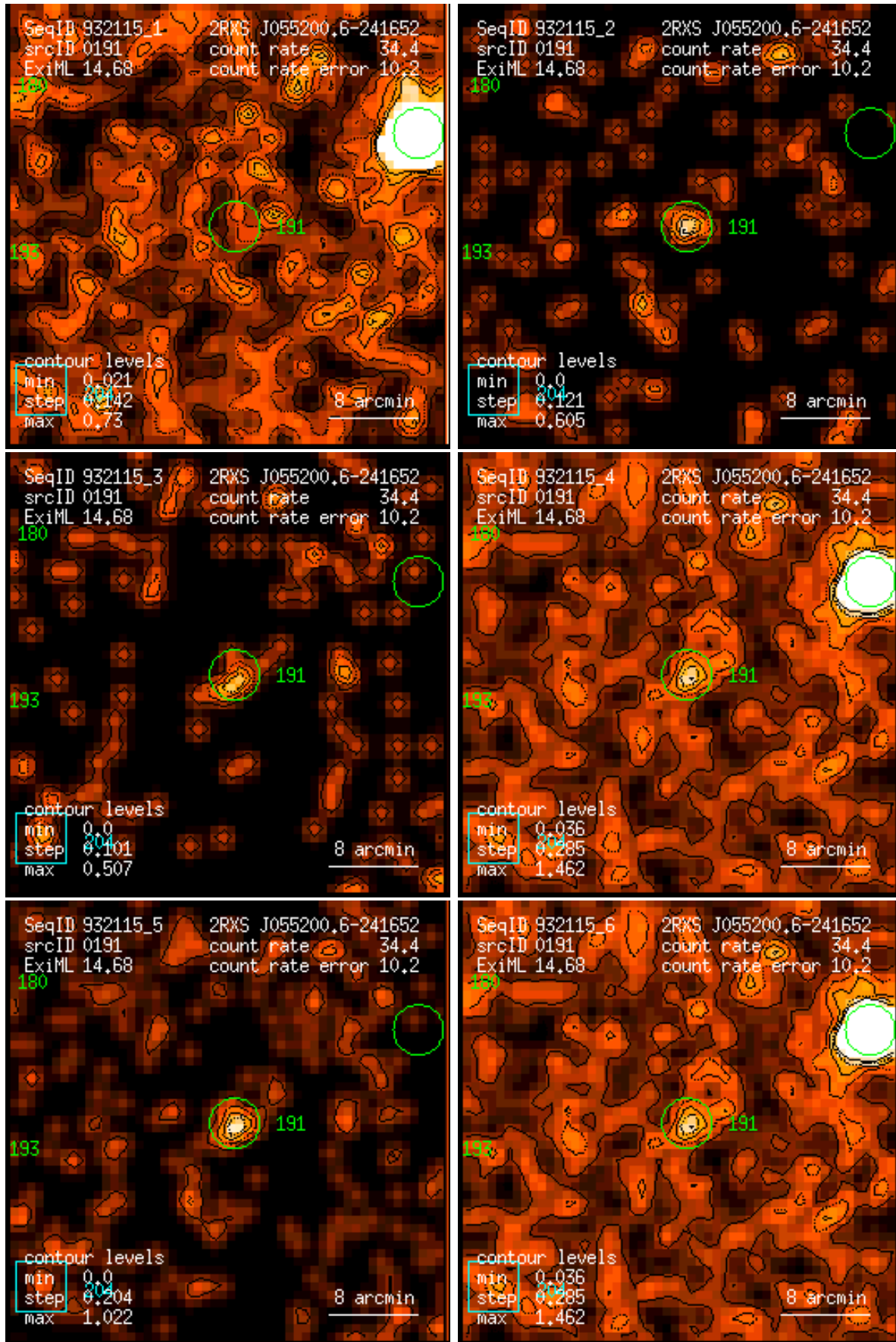
Figure 191: RASS 932115: detection 0191: band rate images, Gaussian filter: (1) PSPC channels 11 – 41, (2) 52 – 90, (3) 91 – 201, (4) 11 – 235, (5) 52 – 201, (6) 11 – 201. Broad band rates in counts/ks. Band rate contour levels in counts/ks/arcmin 2 .
