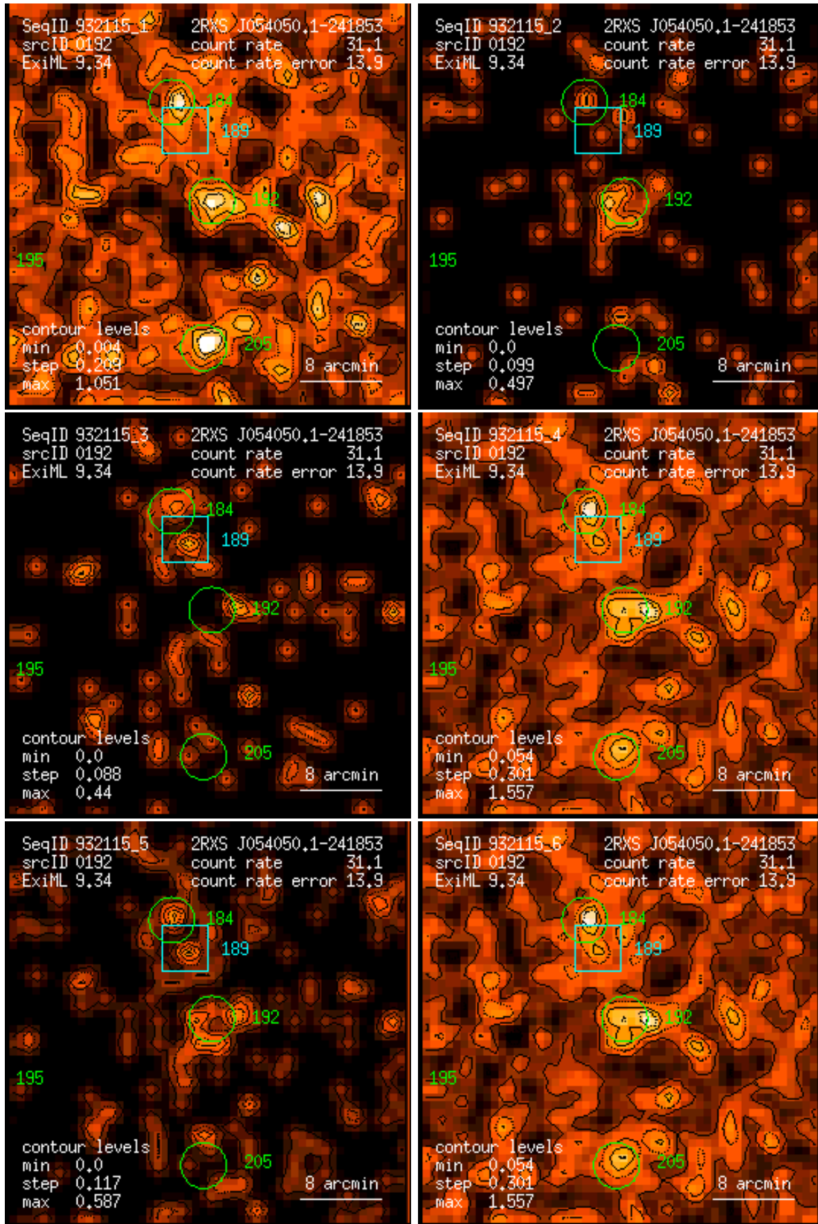
Figure 192: RASS 932115: detection 0192: band rate images, Gaussian filter: (1) PSPC channels 11 – 41, (2) 52 – 90, (3) 91 – 201, (4) 11 – 235, (5) 52 – 201, (6) 11 – 201. Broad band rates in counts/ks. Band rate contour levels in counts/ks/arcmin 2 .
