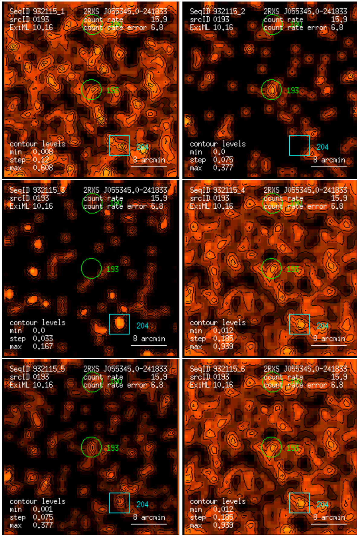
Figure 193: RASS 932115: detection 0193: band rate images, Gaussian filter: (1) PSPC channels 11 – 41, (2) 52 – 90, (3) 91 – 201, (4) 11 – 235, (5) 52 – 201, (6) 11 – 201. Broad band rates in counts/ks. Band rate contour levels in counts/ks/arcmin 2 .
