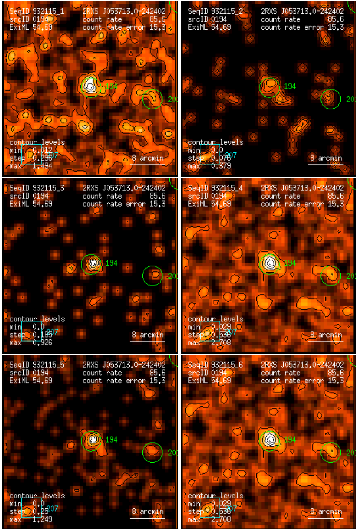
Figure 194: RASS 932115: detection 0194: band rate images, Gaussian filter: (1) PSPC channels 11 – 41, (2) 52 – 90, (3) 91 – 201, (4) 11 – 235, (5) 52 – 201, (6) 11 – 201. Broad band rates in counts/ks. Band rate contour levels in counts/ks/arcmin 2 .
