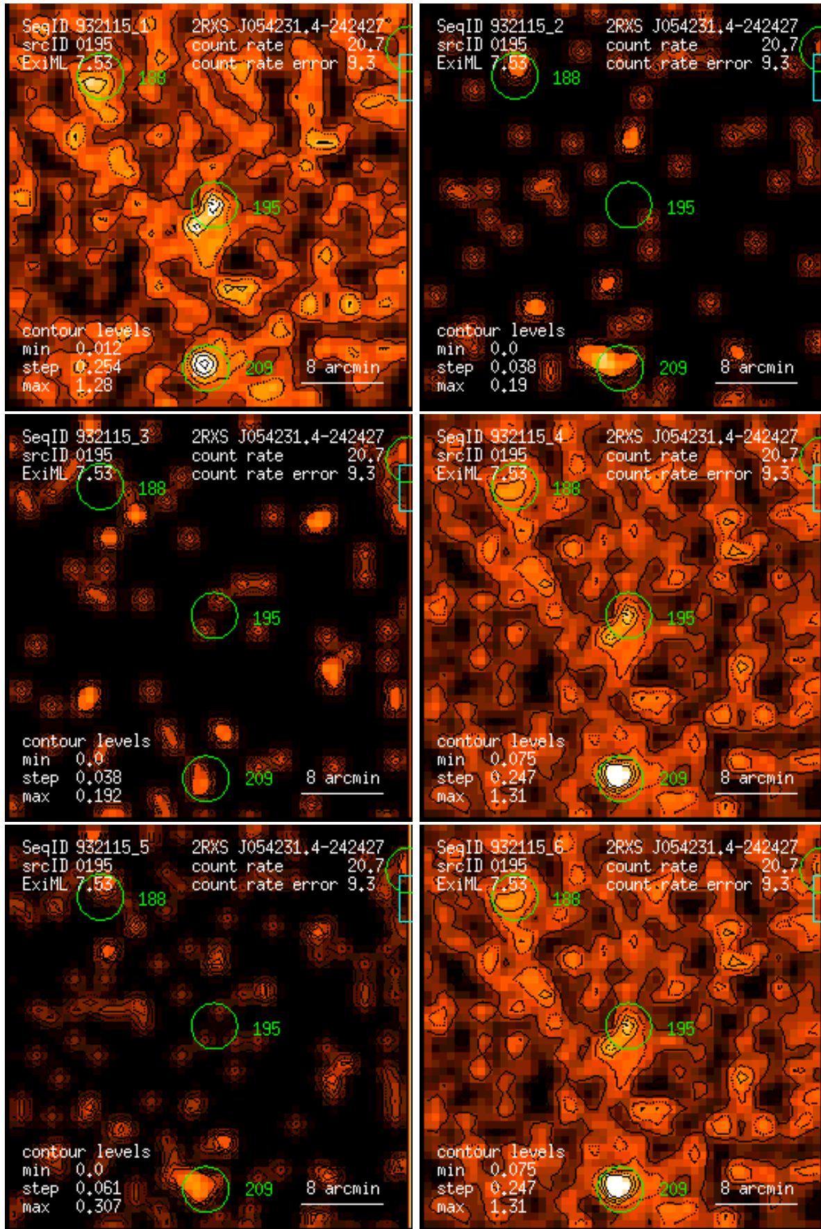
Figure 195: RASS 932115: detection 0195: band rate images, Gaussian filter: (1) PSPC channels 11 – 41, (2) 52 – 90, (3) 91 – 201, (4) 11 – 235, (5) 52 – 201, (6) 11 – 201. Broad band rates in counts/ks. Band rate contour levels in counts/ks/arcmin 2 .
