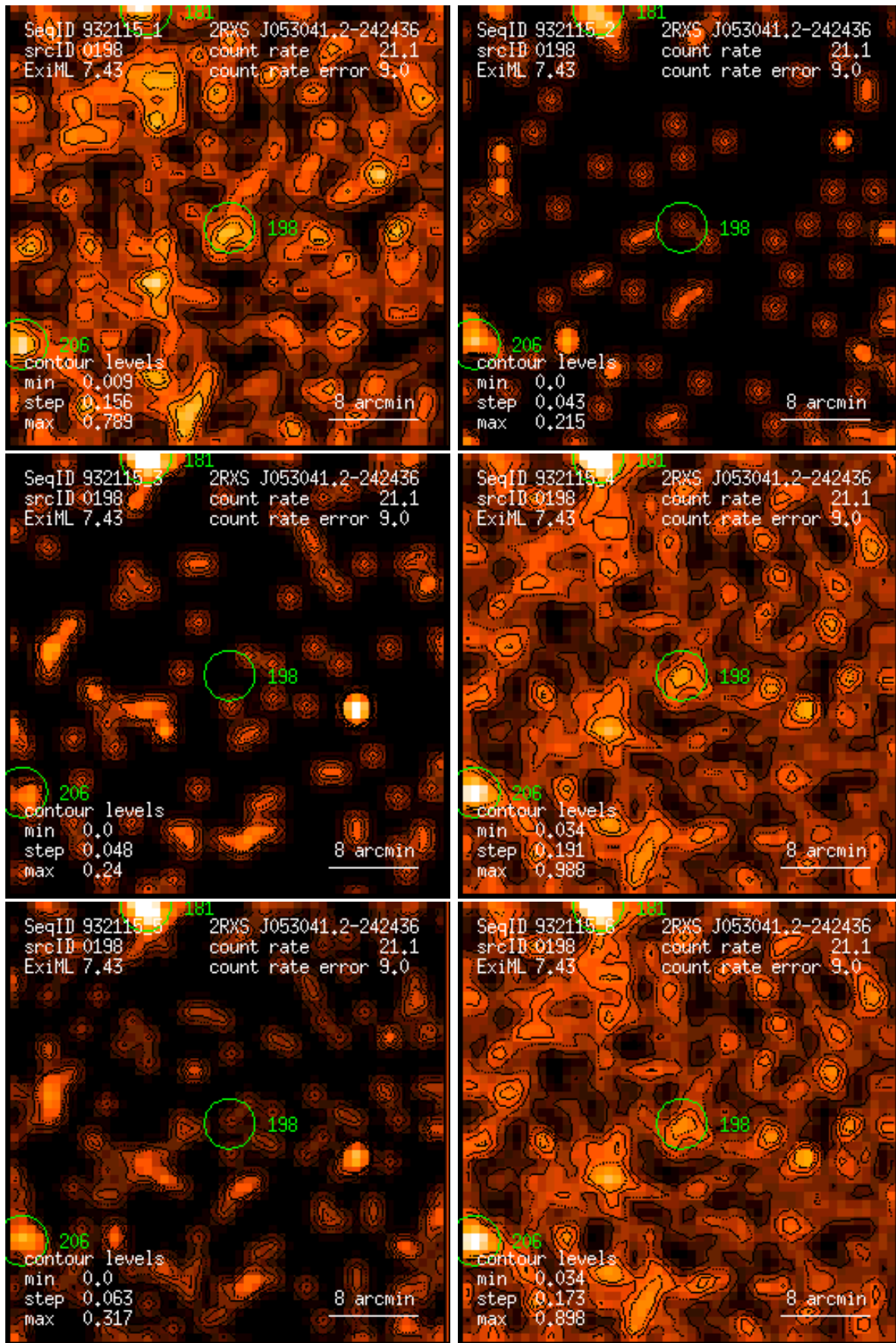
Figure 198: RASS 932115: detection 0198: band rate images, Gaussian filter: (1) PSPC channels 11 – 41, (2) 52 – 90, (3) 91 – 201, (4) 11 – 235, (5) 52 – 201, (6) 11 – 201. Broad band rates in counts/ks. Band rate contour levels in counts/ks/arcmin 2 .
