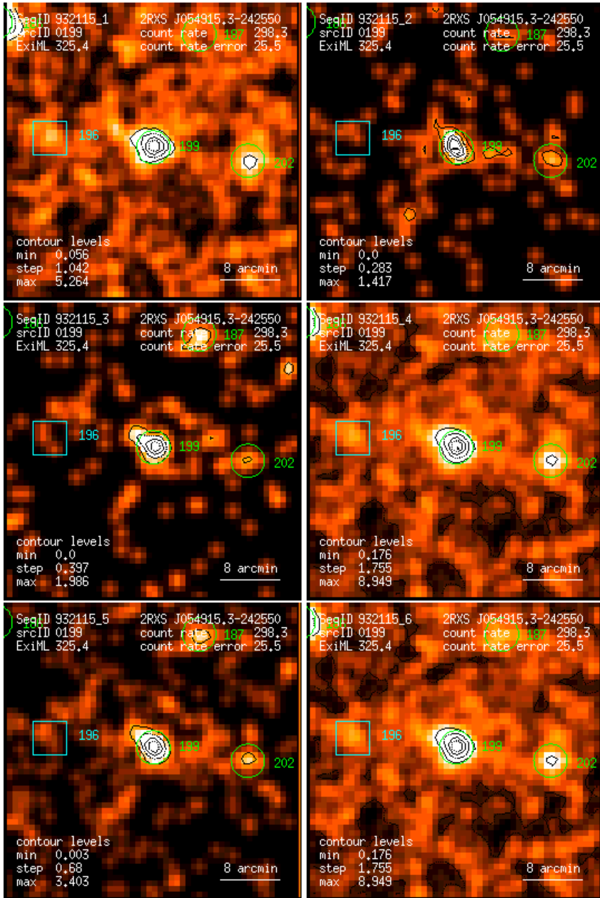
Figure 199: RASS 932115: detection 0199: band rate images, Gaussian filter: (1) PSPC channels 11 – 41, (2) 52 – 90, (3) 91 – 201, (4) 11 – 235, (5) 52 – 201, (6) 11 – 201. Broad band rates in counts/ks. Band rate contour levels in counts/ks/arcmin 2 .
