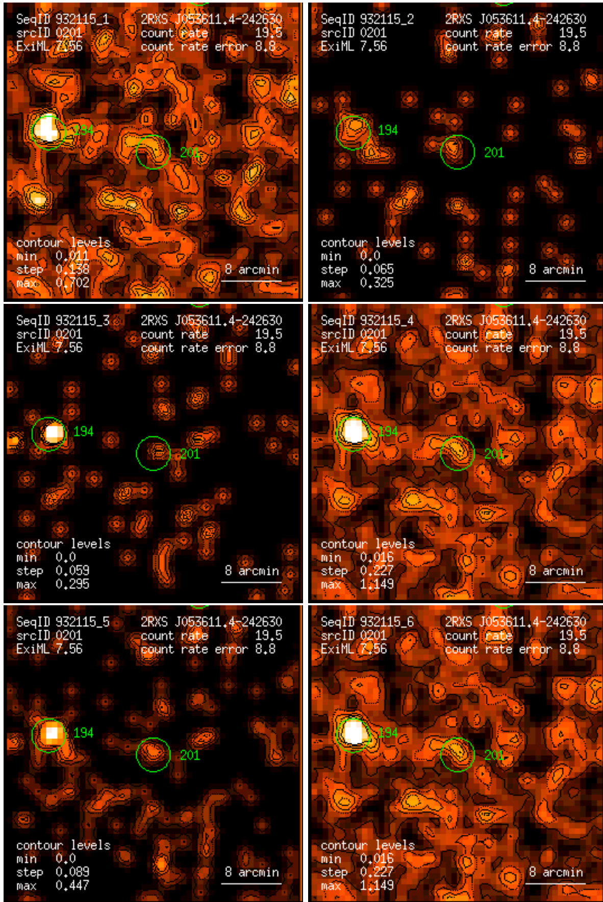
Figure 201: RASS 932115: detection 0201: band rate images, Gaussian filter: (1) PSPC channels 11 – 41, (2) 52 – 90, (3) 91 – 201, (4) 11 – 235, (5) 52 – 201, (6) 11 – 201. Broad band rates in counts/ks. Band rate contour levels in counts/ks/arcmin 2 .
