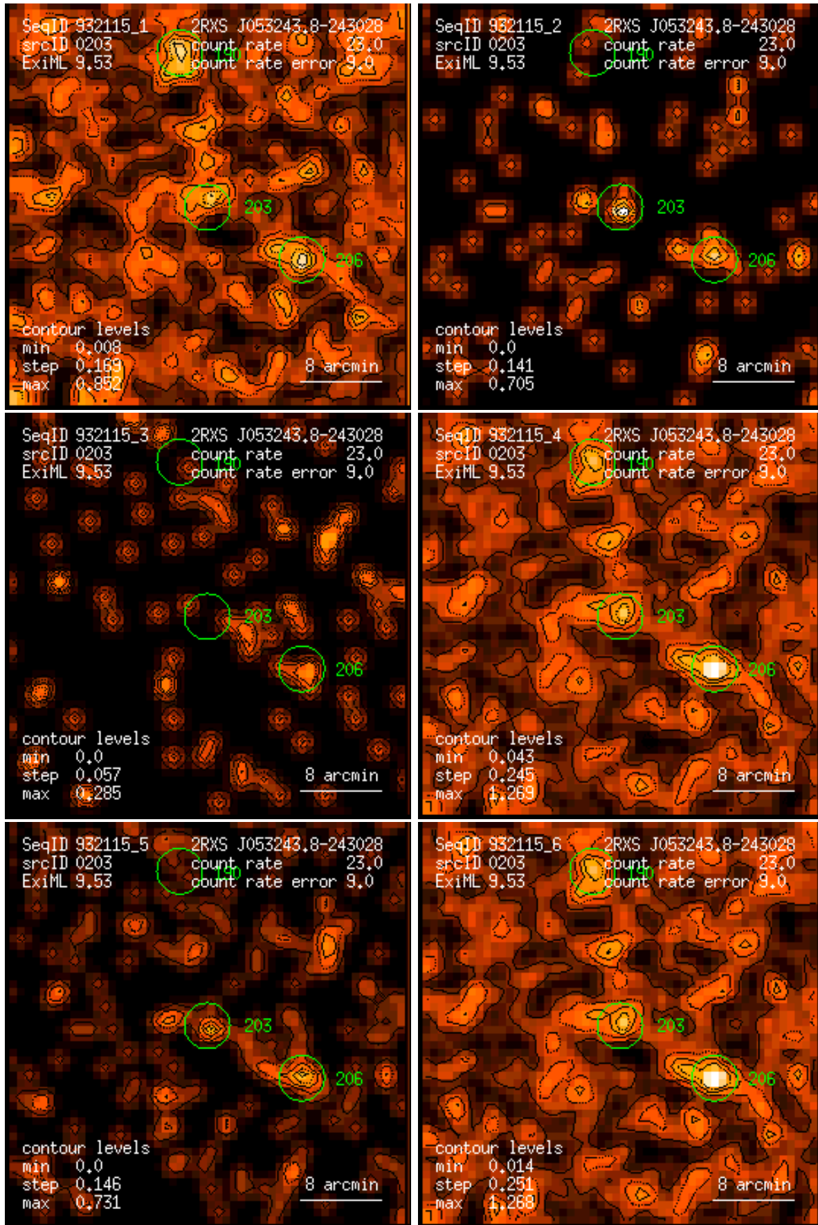
Figure 203: RASS 932115: detection 0203: band rate images, Gaussian filter: (1) PSPC channels 11 – 41, (2) 52 – 90, (3) 91 – 201, (4) 11 – 235, (5) 52 – 201, (6) 11 – 201. Broad band rates in counts/ks. Band rate contour levels in counts/ks/arcmin 2 .
