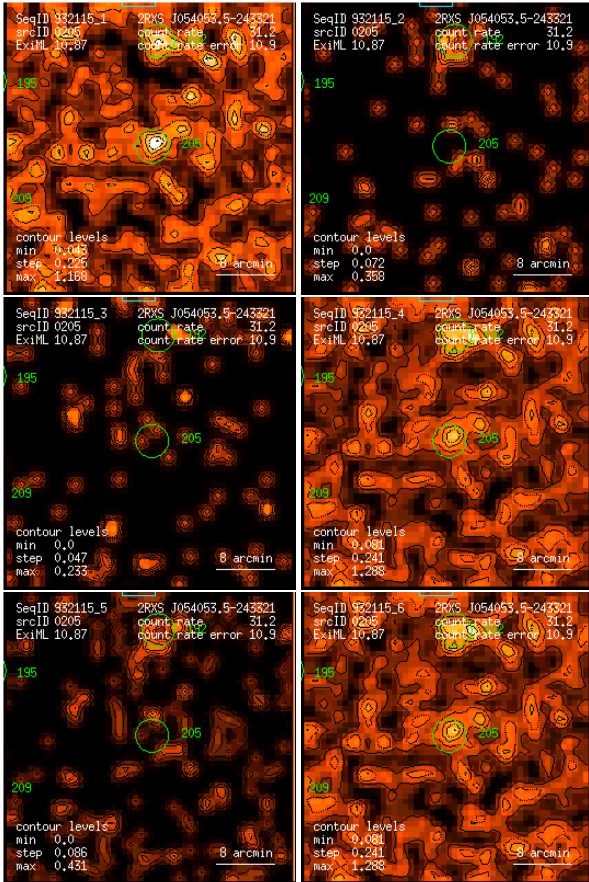
Figure 205: RASS 932115: detection 0205: band rate images, Gaussian filter: (1) PSPC channels 11 – 41, (2) 52 – 90, (3) 91 – 201, (4) 11 – 235, (5) 52 – 201, (6) 11 – 201. Broad band rates in counts/ks. Band rate contour levels in counts/ks/arcmin 2 .
