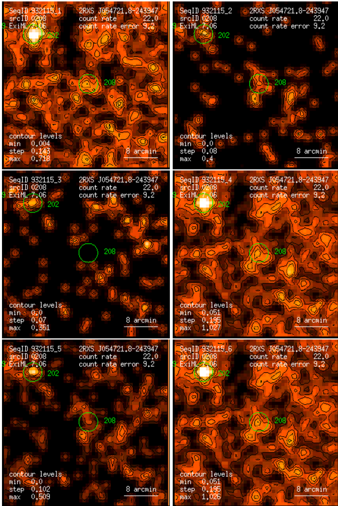
Figure 208: RASS 932115: detection 0208: band rate images, Gaussian filter: (1) PSPC channels 11 – 41, (2) 52 – 90, (3) 91 – 201, (4) 11 – 235, (5) 52 – 201, (6) 11 – 201. Broad band rates in counts/ks. Band rate contour levels in counts/ks/arcmin 2 .
