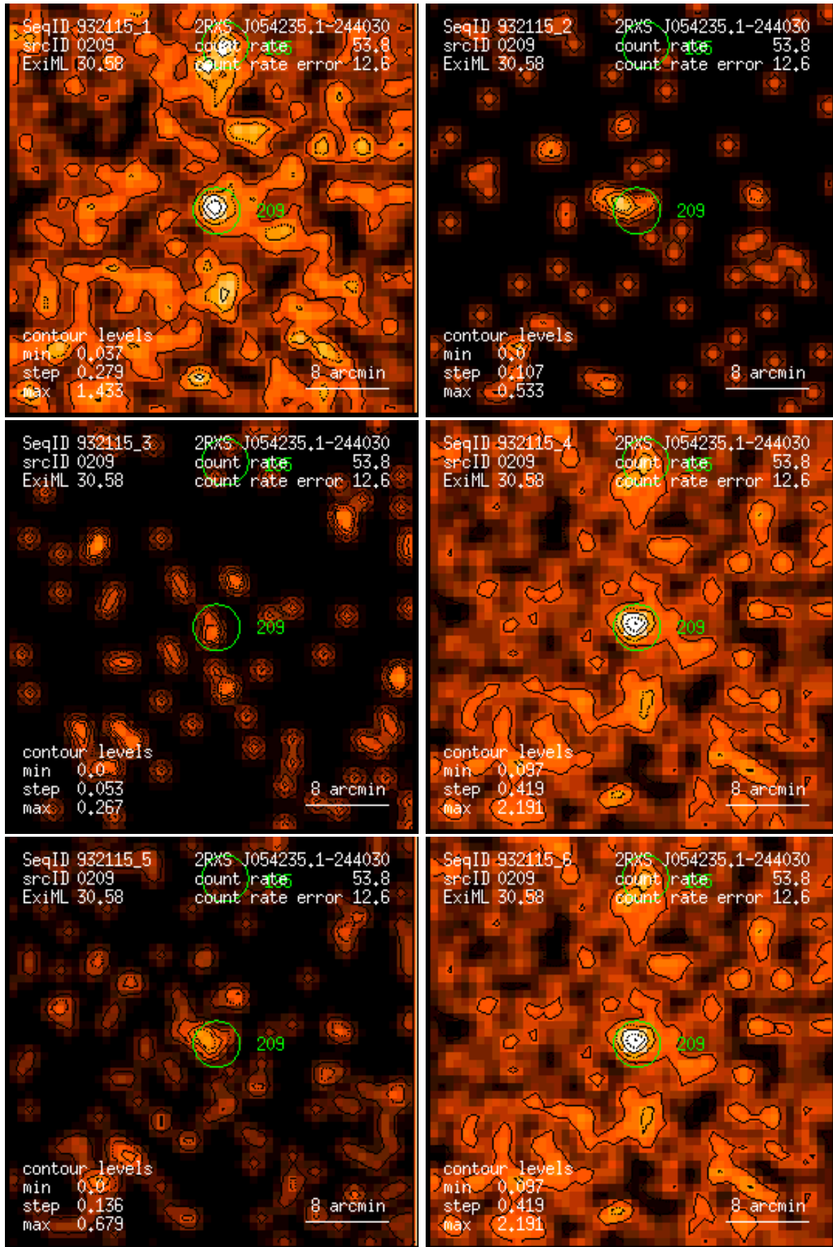
Figure 209: RASS 932115: detection 0209: band rate images, Gaussian filter: (1) PSPC channels 11 – 41, (2) 52 – 90, (3) 91 – 201, (4) 11 – 235, (5) 52 – 201, (6) 11 – 201. Broad band rates in counts/ks. Band rate contour levels in counts/ks/arcmin 2 .
