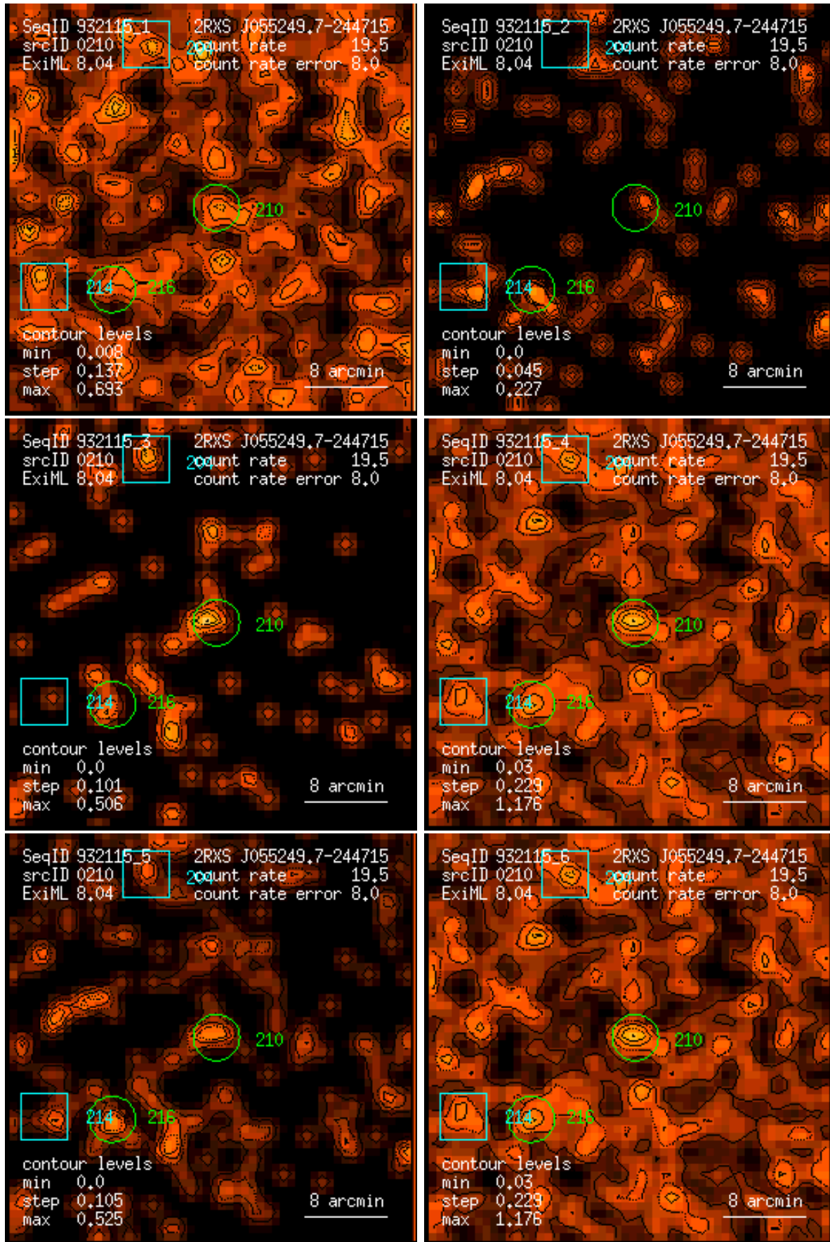
Figure 210: RASS 932115: detection 0210: band rate images, Gaussian filter: (1) PSPC channels 11 – 41, (2) 52 – 90, (3) 91 – 201, (4) 11 – 235, (5) 52 – 201, (6) 11 – 201. Broad band rates in counts/ks. Band rate contour levels in counts/ks/arcmin 2 .
