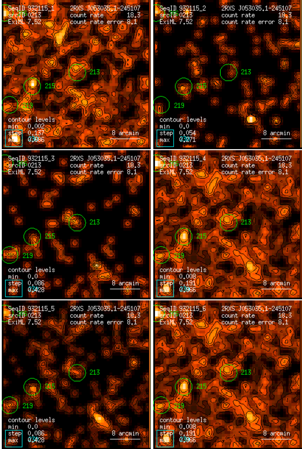
Figure 213: RASS 932115: detection 0213: band rate images, Gaussian filter: (1) PSPC channels 11 – 41, (2) 52 – 90, (3) 91 – 201, (4) 11 – 235, (5) 52 – 201, (6) 11 – 201. Broad band rates in counts/ks. Band rate contour levels in counts/ks/arcmin 2 .
