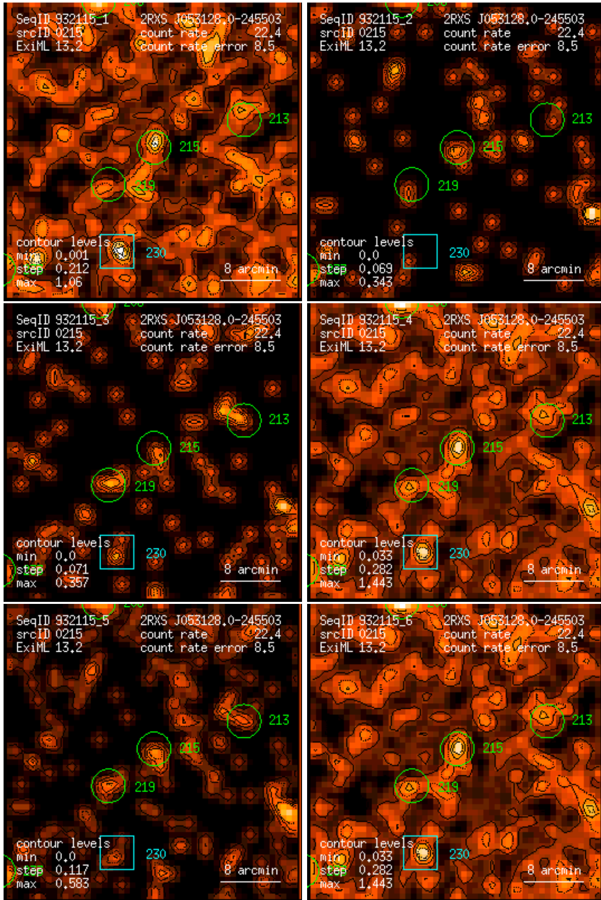
Figure 215: RASS 932115: detection 0215: band rate images, Gaussian filter: (1) PSPC channels 11 – 41, (2) 52 – 90, (3) 91 – 201, (4) 11 – 235, (5) 52 – 201, (6) 11 – 201. Broad band rates in counts/ks. Band rate contour levels in counts/ks/arcmin 2 .
