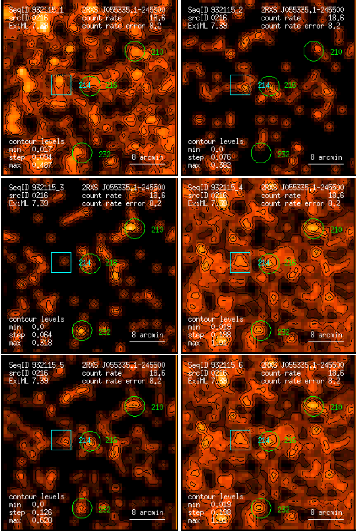
Figure 216: RASS 932115: detection 0216: band rate images, Gaussian filter: (1) PSPC channels 11 – 41, (2) 52 – 90, (3) 91 – 201, (4) 11 – 235, (5) 52 – 201, (6) 11 – 201. Broad band rates in counts/ks. Band rate contour levels in counts/ks/arcmin 2 .
