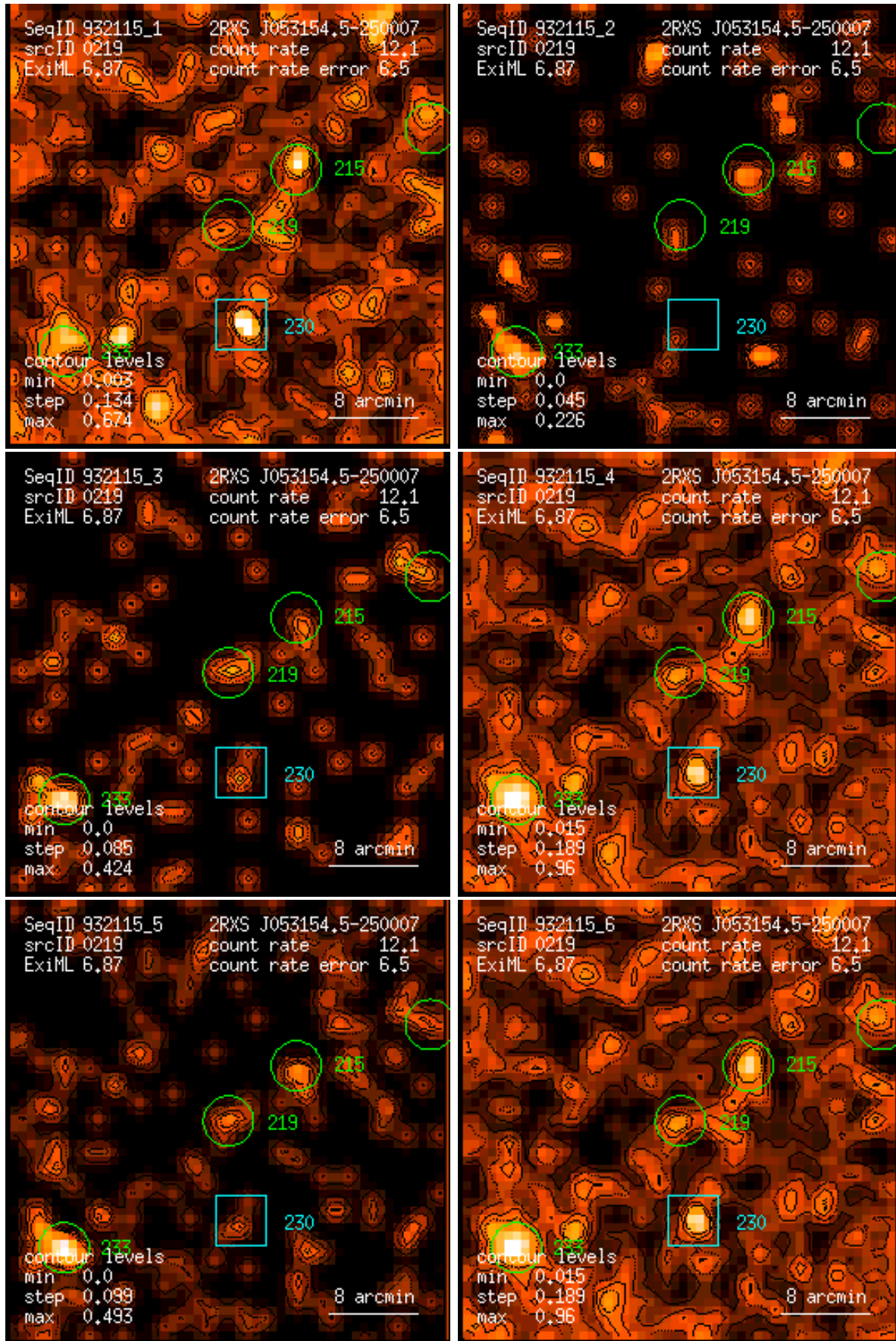
Figure 219: RASS 932115: detection 0219: band rate images, Gaussian filter: (1) PSPC channels 11 – 41, (2) 52 – 90, (3) 91 – 201, (4) 11 – 235, (5) 52 – 201, (6) 11 – 201. Broad band rates in counts/ks. Band rate contour levels in counts/ks/arcmin 2 .
