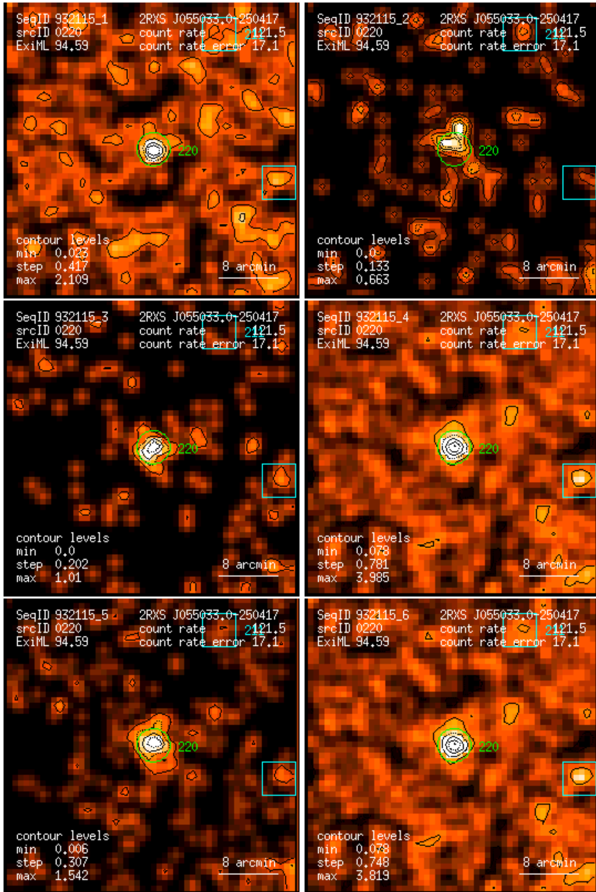
Figure 220: RASS 932115: detection 0220: band rate images, Gaussian filter: (1) PSPC channels 11 – 41, (2) 52 – 90, (3) 91 – 201, (4) 11 – 235, (5) 52 – 201, (6) 11 – 201. Broad band rates in counts/ks. Band rate contour levels in counts/ks/arcmin 2 .
