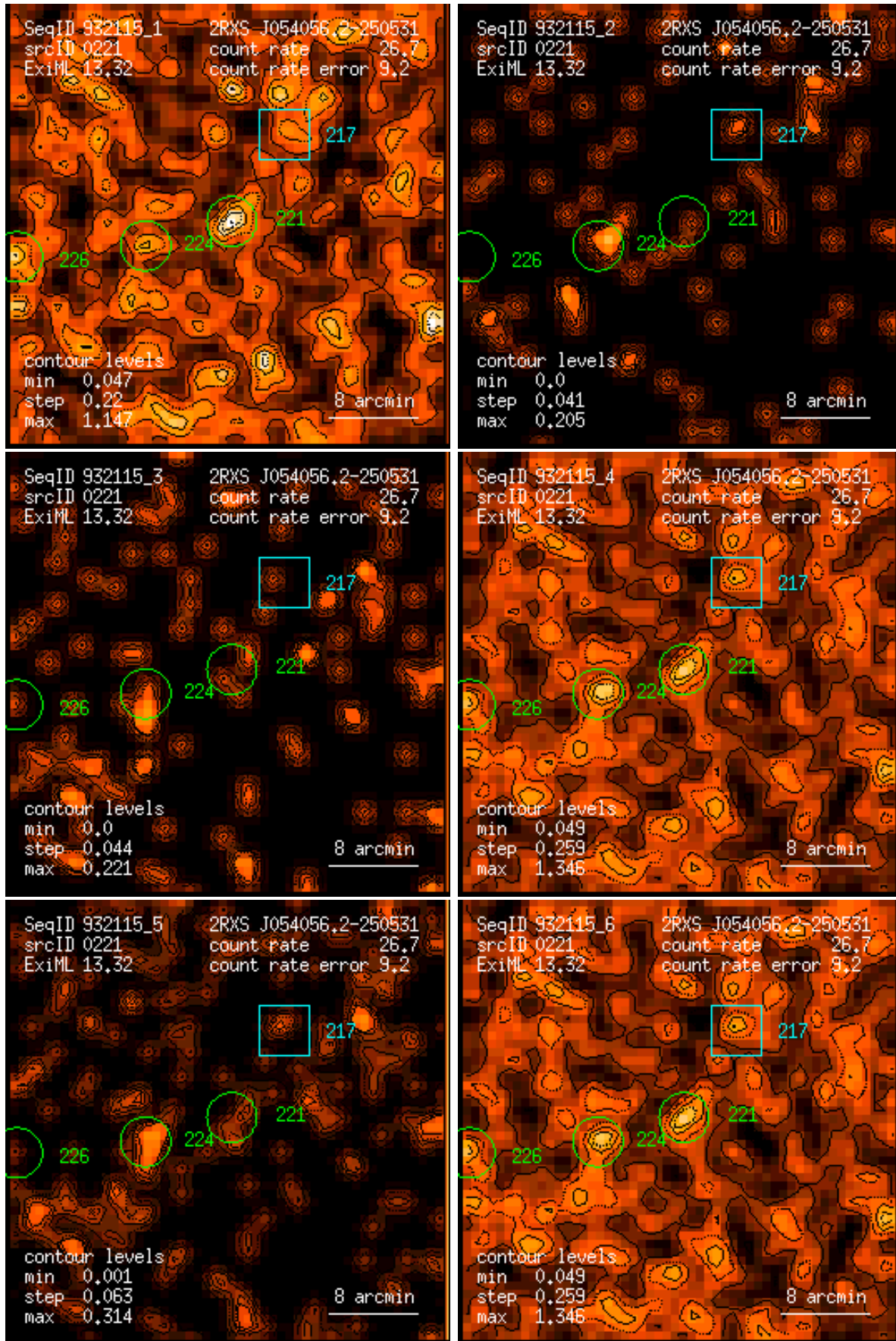
Figure 221: RASS 932115: detection 0221: band rate images, Gaussian filter: (1) PSPC channels 11 – 41, (2) 52 – 90, (3) 91 – 201, (4) 11 – 235, (5) 52 – 201, (6) 11 – 201. Broad band rates in counts/ks. Band rate contour levels in counts/ks/arcmin 2 .
