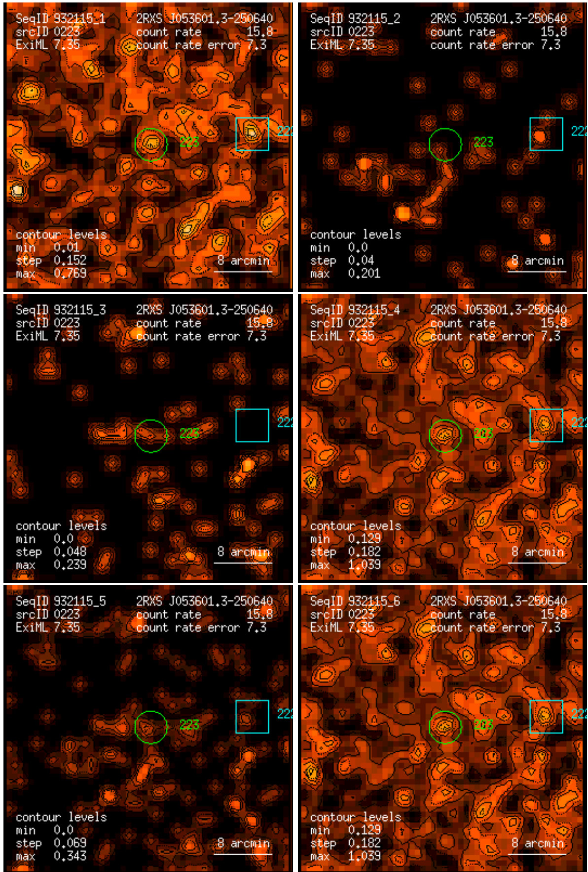
Figure 223: RASS 932115: detection 0223: band rate images, Gaussian filter: (1) PSPC channels 11 – 41, (2) 52 – 90, (3) 91 – 201, (4) 11 – 235, (5) 52 – 201, (6) 11 – 201. Broad band rates in counts/ks. Band rate contour levels in counts/ks/arcmin 2 .
