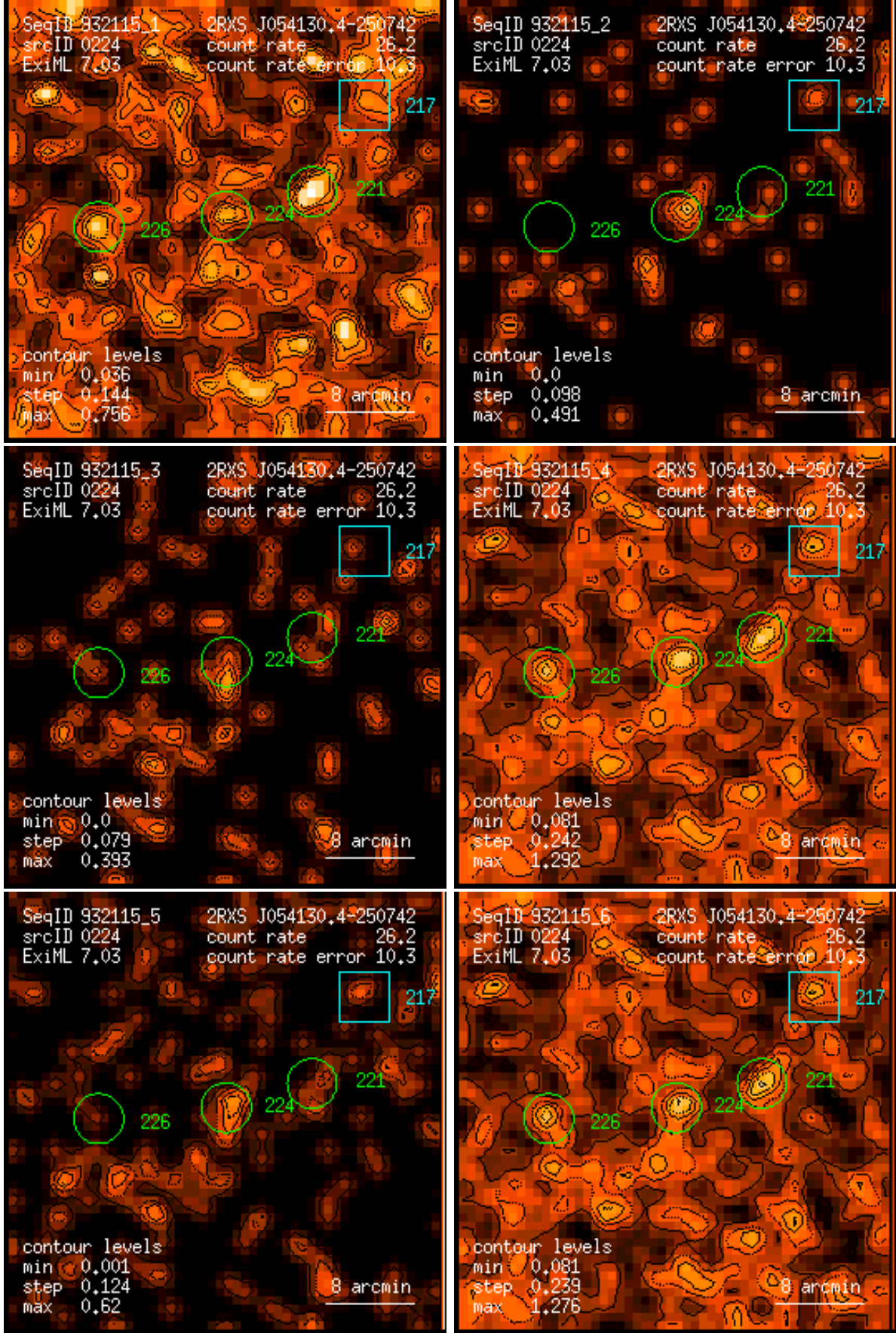
Figure 224: RASS 932115: detection 0224: band rate images, Gaussian filter: (1) PSPC channels 11 – 41, (2) 52 – 90, (3) 91 – 201, (4) 11 – 235, (5) 52 – 201, (6) 11 – 201. Broad band rates in counts/ks. Band rate contour levels in counts/ks/arcmin 2 .
