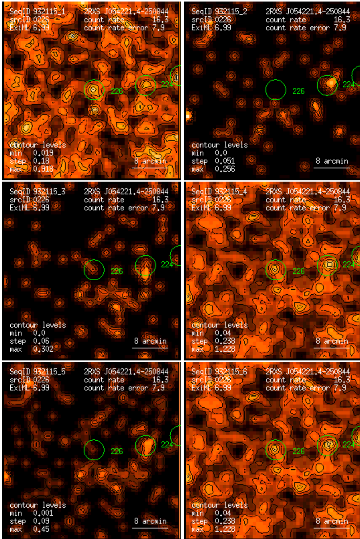
Figure 226: RASS 932115: detection 0226: band rate images, Gaussian filter: (1) PSPC channels 11 – 41, (2) 52 – 90, (3) 91 – 201, (4) 11 – 235, (5) 52 – 201, (6) 11 – 201. Broad band rates in counts/ks. Band rate contour levels in counts/ks/arcmin 2 .
