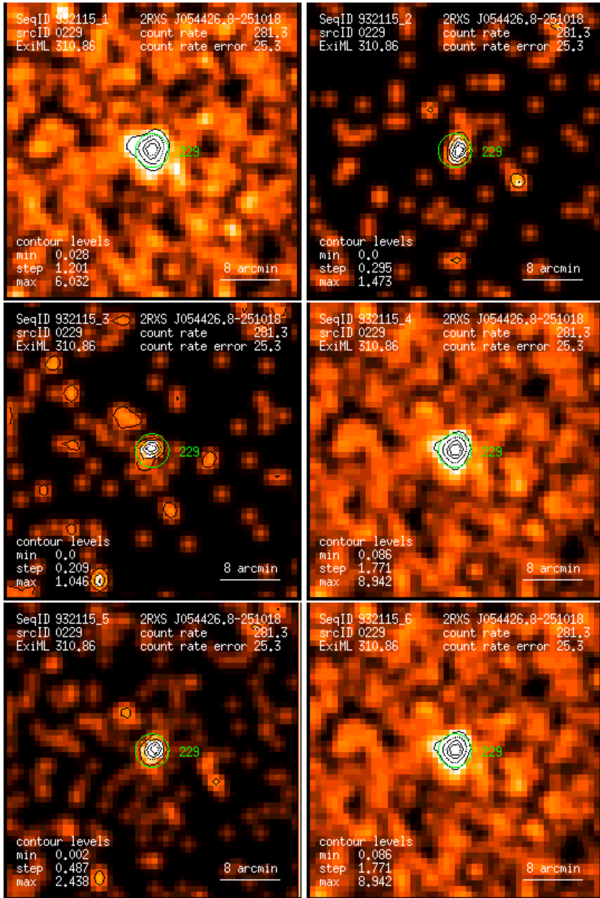
Figure 229: RASS 932115: detection 0229: band rate images, Gaussian filter: (1) PSPC channels 11 – 41, (2) 52 – 90, (3) 91 – 201, (4) 11 – 235, (5) 52 – 201, (6) 11 – 201. Broad band rates in counts/ks. Band rate contour levels in counts/ks/arcmin 2 .
