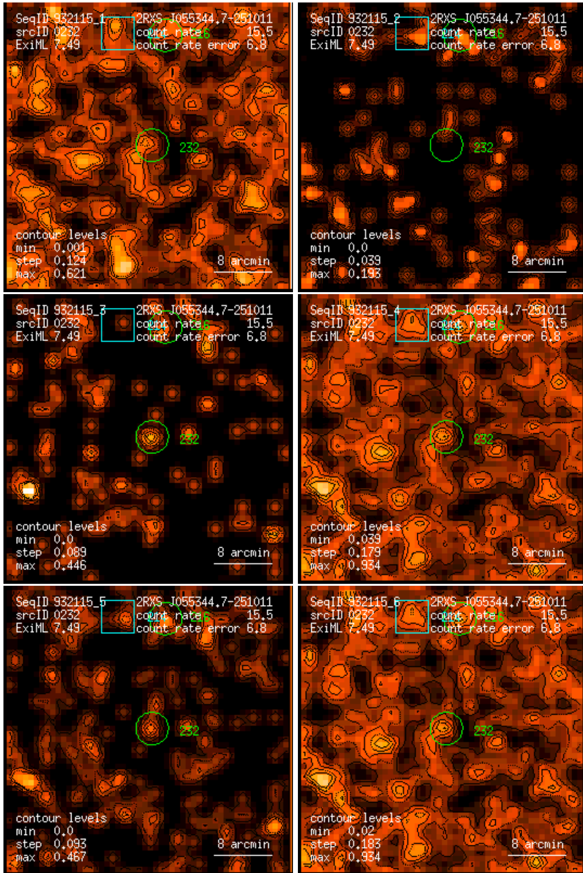
Figure 232: RASS 932115: detection 0232: band rate images, Gaussian filter: (1) PSPC channels 11 – 41, (2) 52 – 90, (3) 91 – 201, (4) 11 – 235, (5) 52 – 201, (6) 11 – 201. Broad band rates in counts/ks. Band rate contour levels in counts/ks/arcmin 2 .
