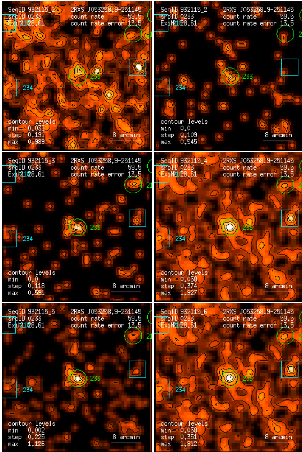
Figure 233: RASS 932115: detection 0233: band rate images, Gaussian filter: (1) PSPC channels 11 – 41, (2) 52 – 90, (3) 91 – 201, (4) 11 – 235, (5) 52 – 201, (6) 11 – 201. Broad band rates in counts/ks. Band rate contour levels in counts/ks/arcmin 2 .
