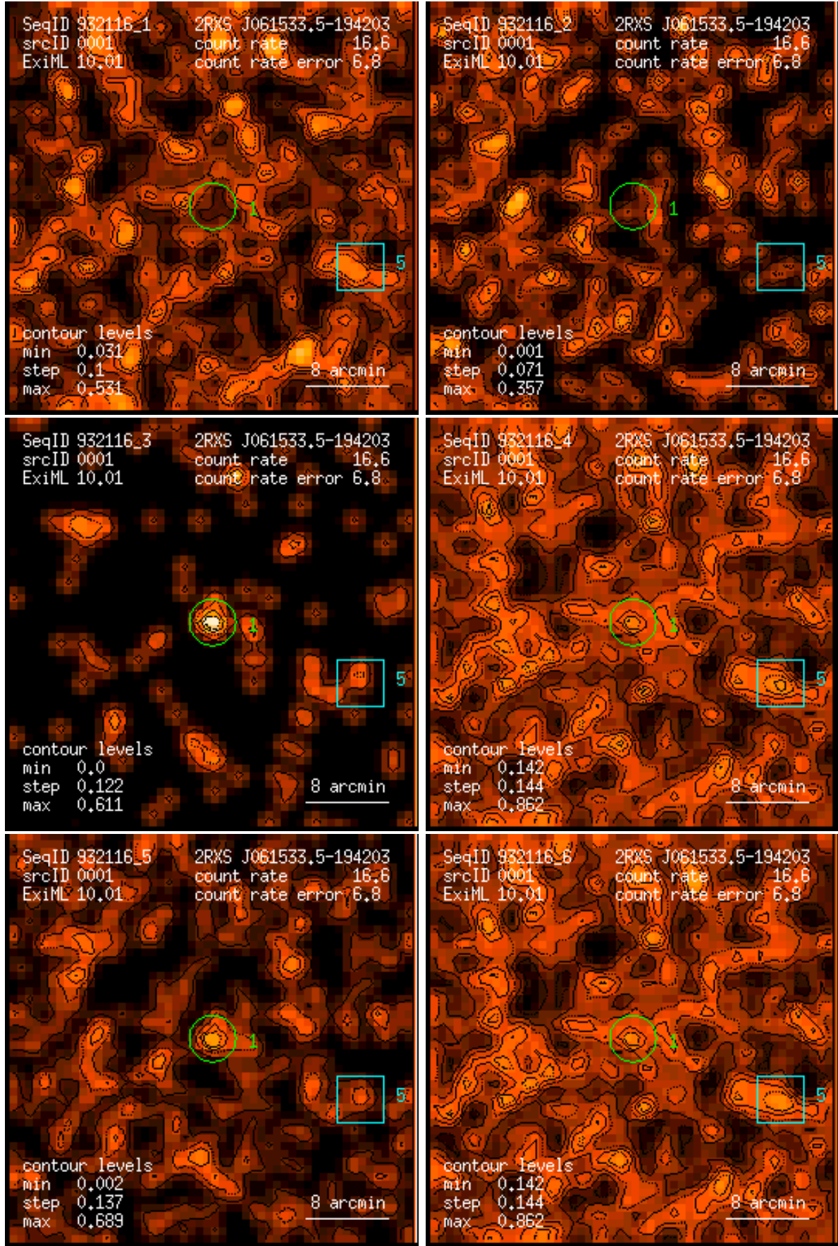
Figure 1: RASS 932116: detection 0001: band rate images, Gaussian filter: (1) PSPC channels 11 – 41, (2) 52 – 90, (3) 91 – 201, (4) 11 – 235, (5) 52 – 201, (6) 11 – 201. Broad band rates in counts/ks. Band rate contour levels in counts/ks/arcmin 2 .
