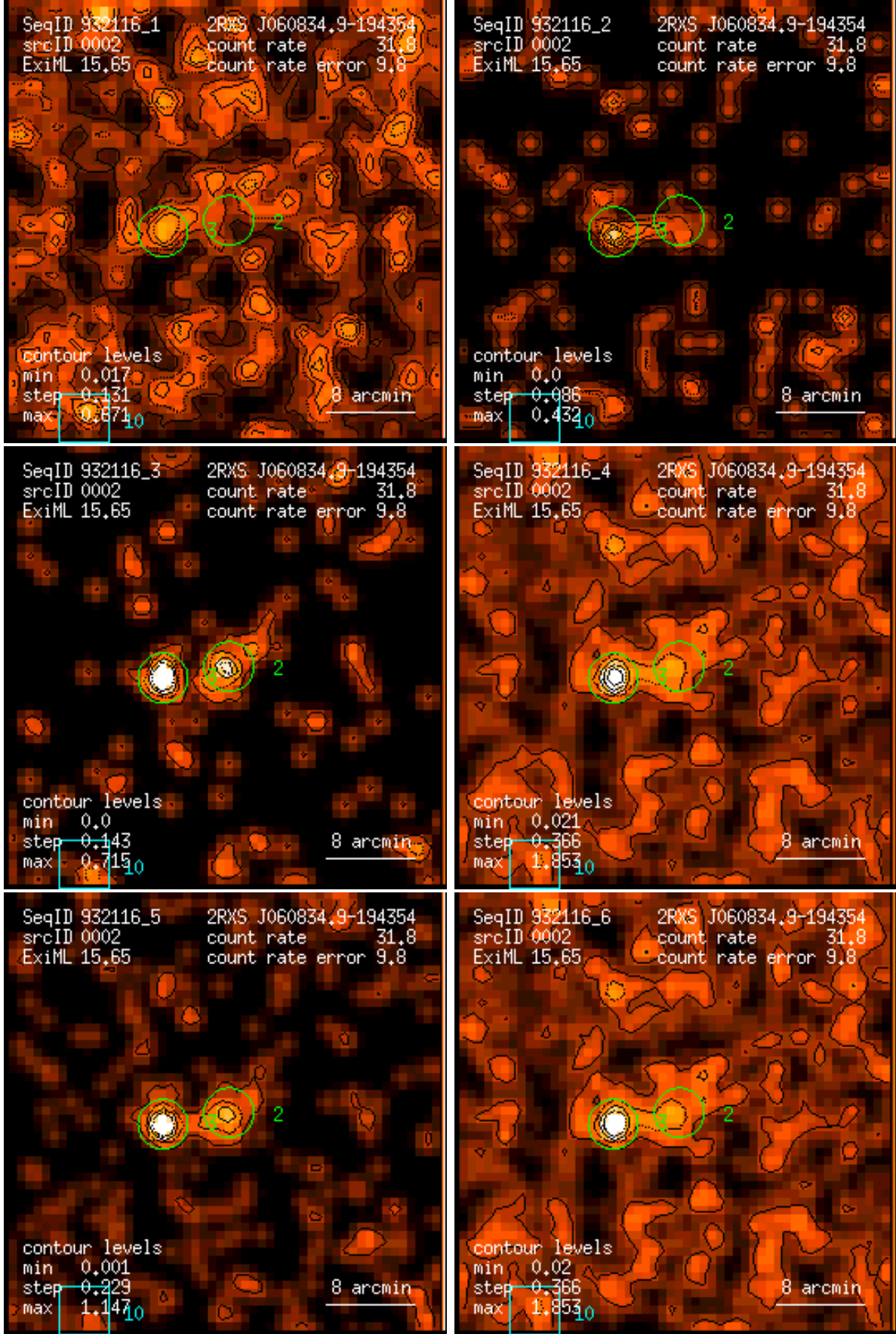
Figure 2: RASS 932116: detection 0002: band rate images, Gaussian filter: (1) PSPC channels 11 – 41, (2) 52 – 90, (3) 91 – 201, (4) 11 – 235, (5) 52 – 201, (6) 11 – 201. Broad band rates in counts/ks. Band rate contour levels in counts/ks/arcmin 2 .
