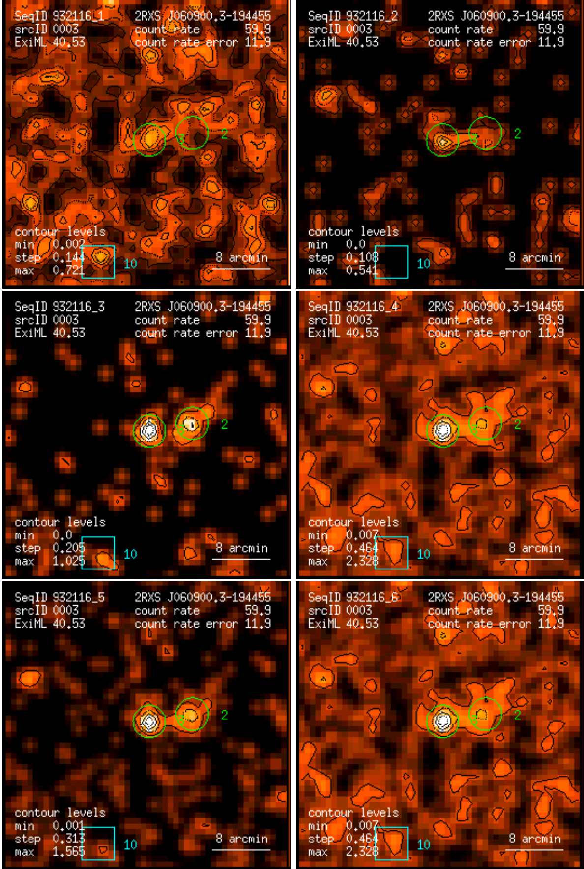
Figure 3: RASS 932116: detection 0003: band rate images, Gaussian filter: (1) PSPC channels 11 – 41, (2) 52 – 90, (3) 91 – 201, (4) 11 – 235, (5) 52 – 201, (6) 11 – 201. Broad band rates in counts/ks. Band rate contour levels in counts/ks/arcmin 2 .
