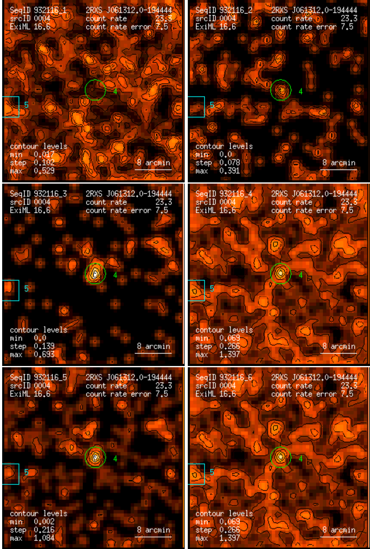
Figure 4: RASS 932116: detection 0004: band rate images, Gaussian filter: (1) PSPC channels 11 – 41, (2) 52 – 90, (3) 91 – 201, (4) 11 – 235, (5) 52 – 201, (6) 11 – 201. Broad band rates in counts/ks. Band rate contour levels in counts/ks/arcmin 2 .
